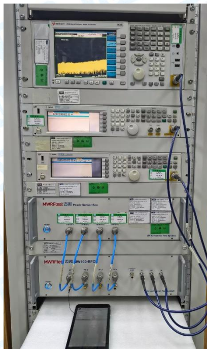
Photo of Setup for Conducted Measurements
