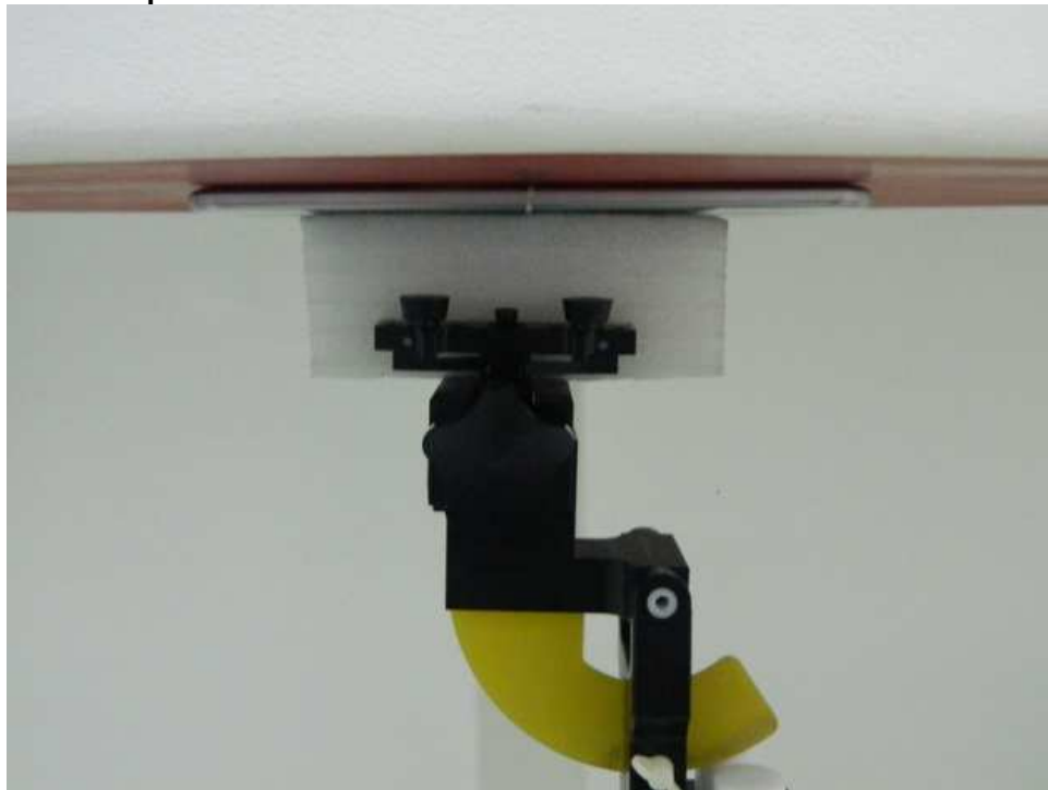
Photograph 2: Set-up for Edge 1
