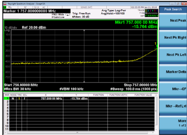
ANT- Vertical756.9-757MHz
