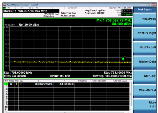
ANT- Horizontal758-758.1MHz
