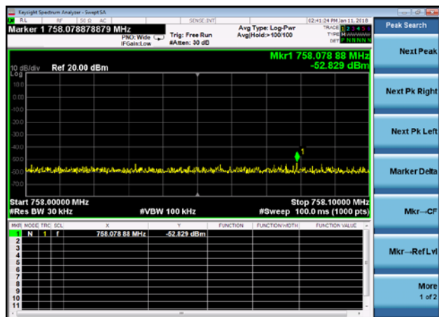
ANT- Vertical758-758.1MHz
