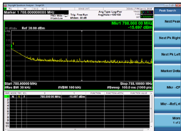
ANT- Vertical788.0-788.1MHz
