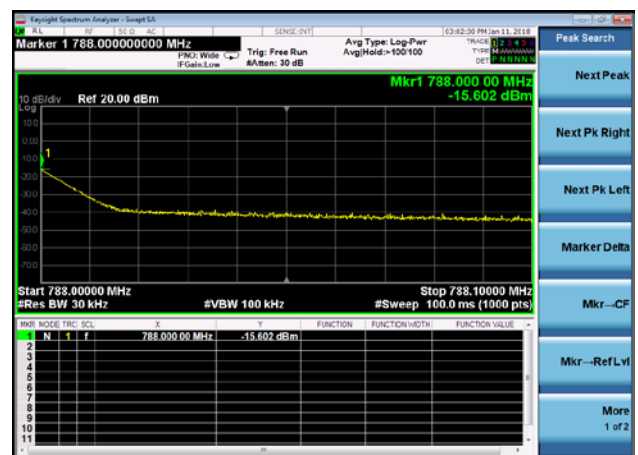
ANT- Horizontal788.0-788.1MHz
