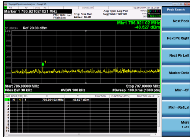
ANT- Vertical786.9-787MHz
