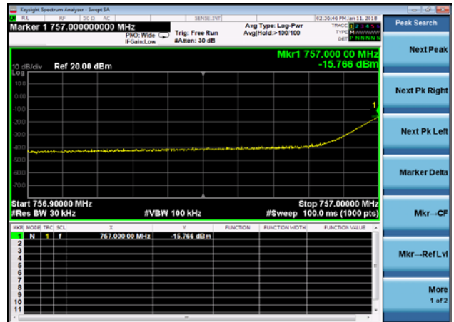
ANT- Horizontal756.9-757MHz
