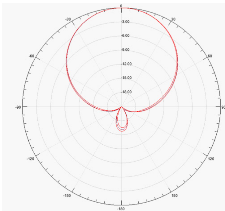
Radiation pattern M Plane 440MHz, 455MHz & 470MHz
