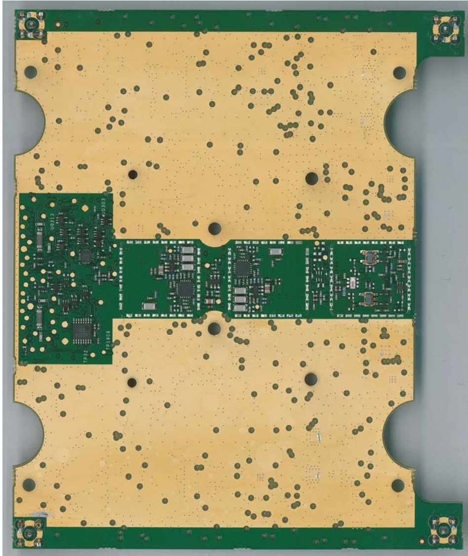
RF_BOARD_BOT_NO_SHIELDS
