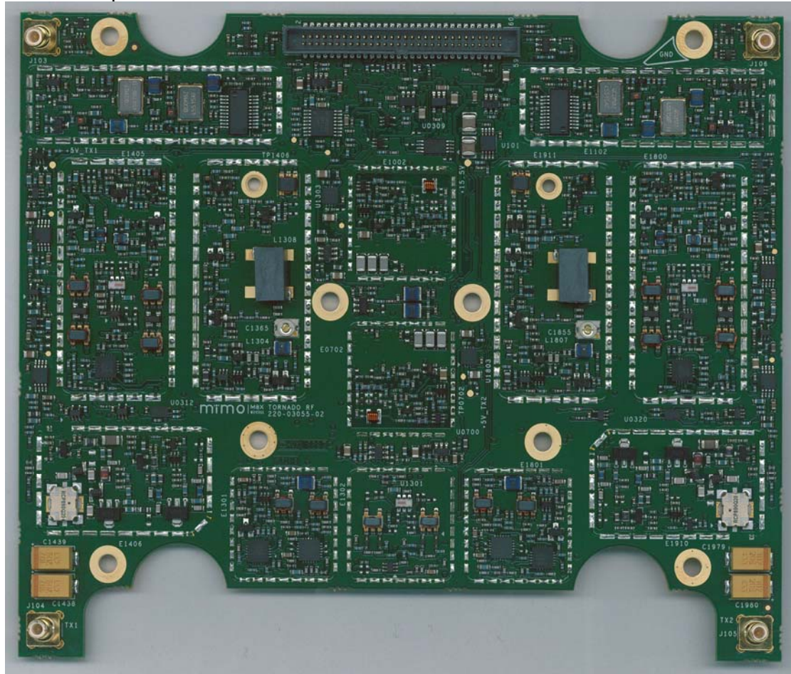
RF board top with shields
