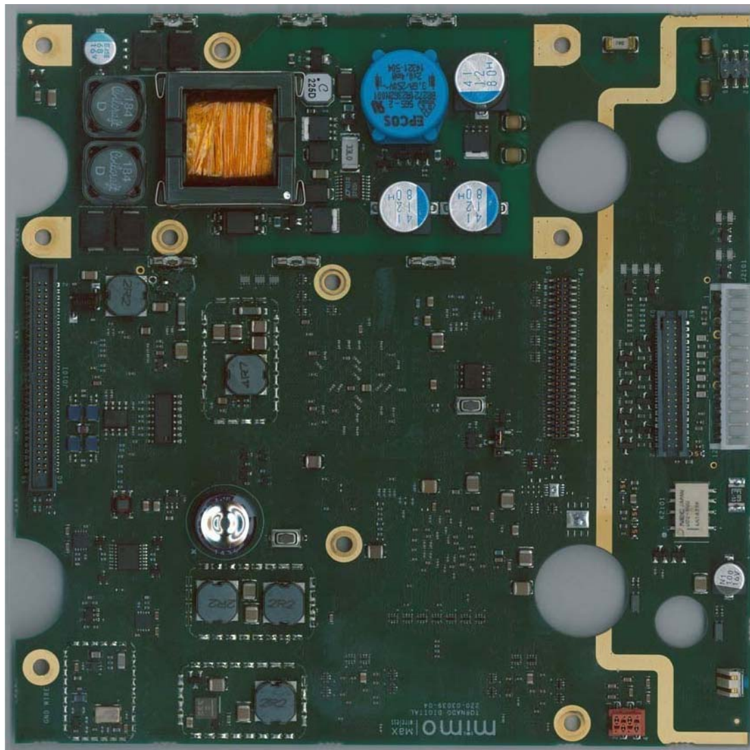
Digital board top side no shields
