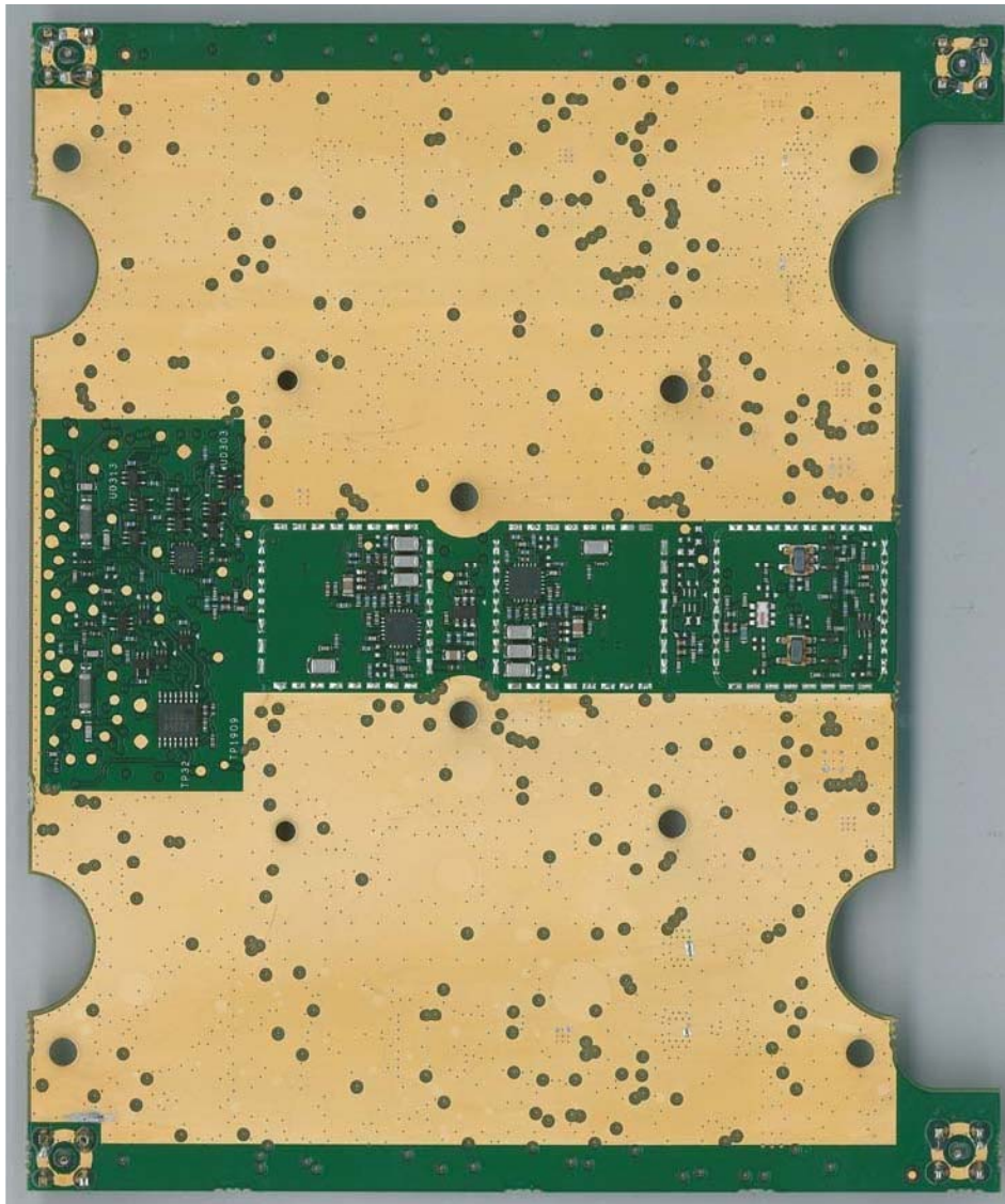
RF board bottom side no shields
