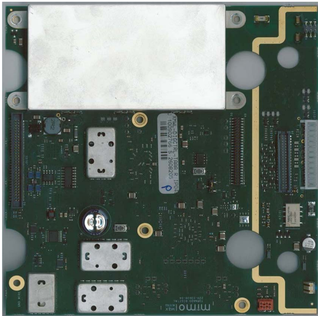
Digital board top side with shields
