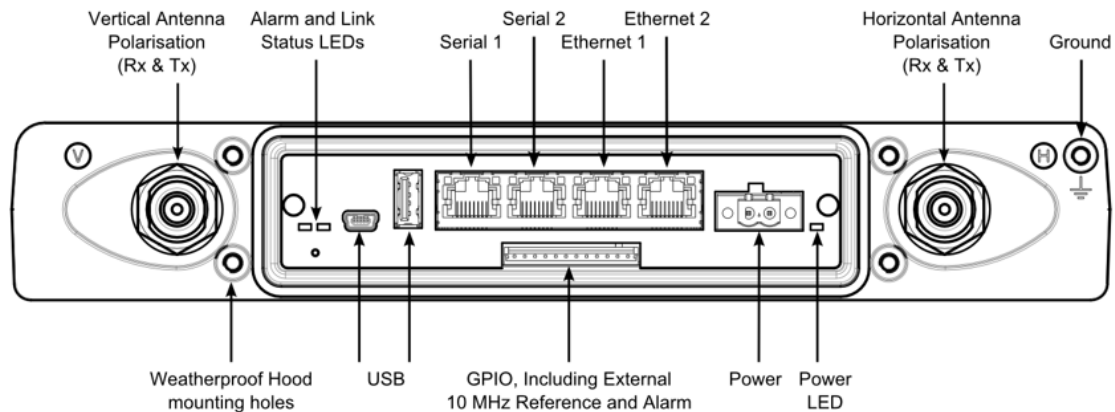
Connectors
