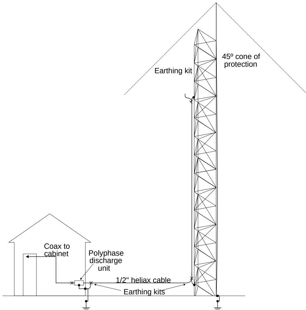
Lightning protection
