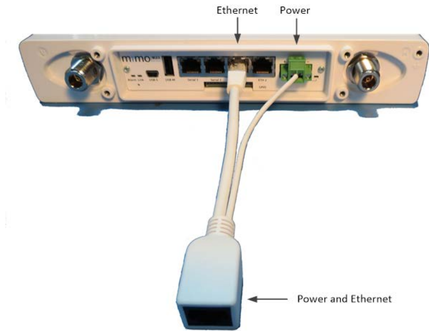
PoE Splitter
