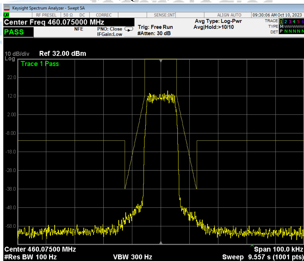
Port-V/256QAM/12.5 kHz/Mask D
