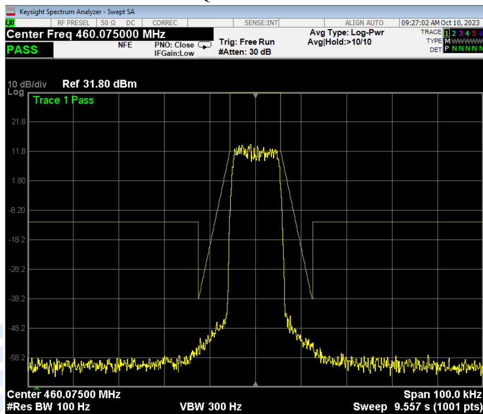
Port-V/64QAM/12.5 kHz/Mask D
