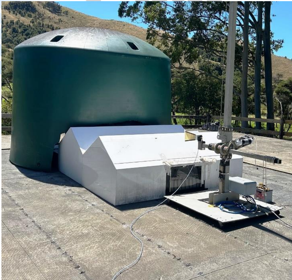
Horn Antenna pointing towards Test Enclosure.
