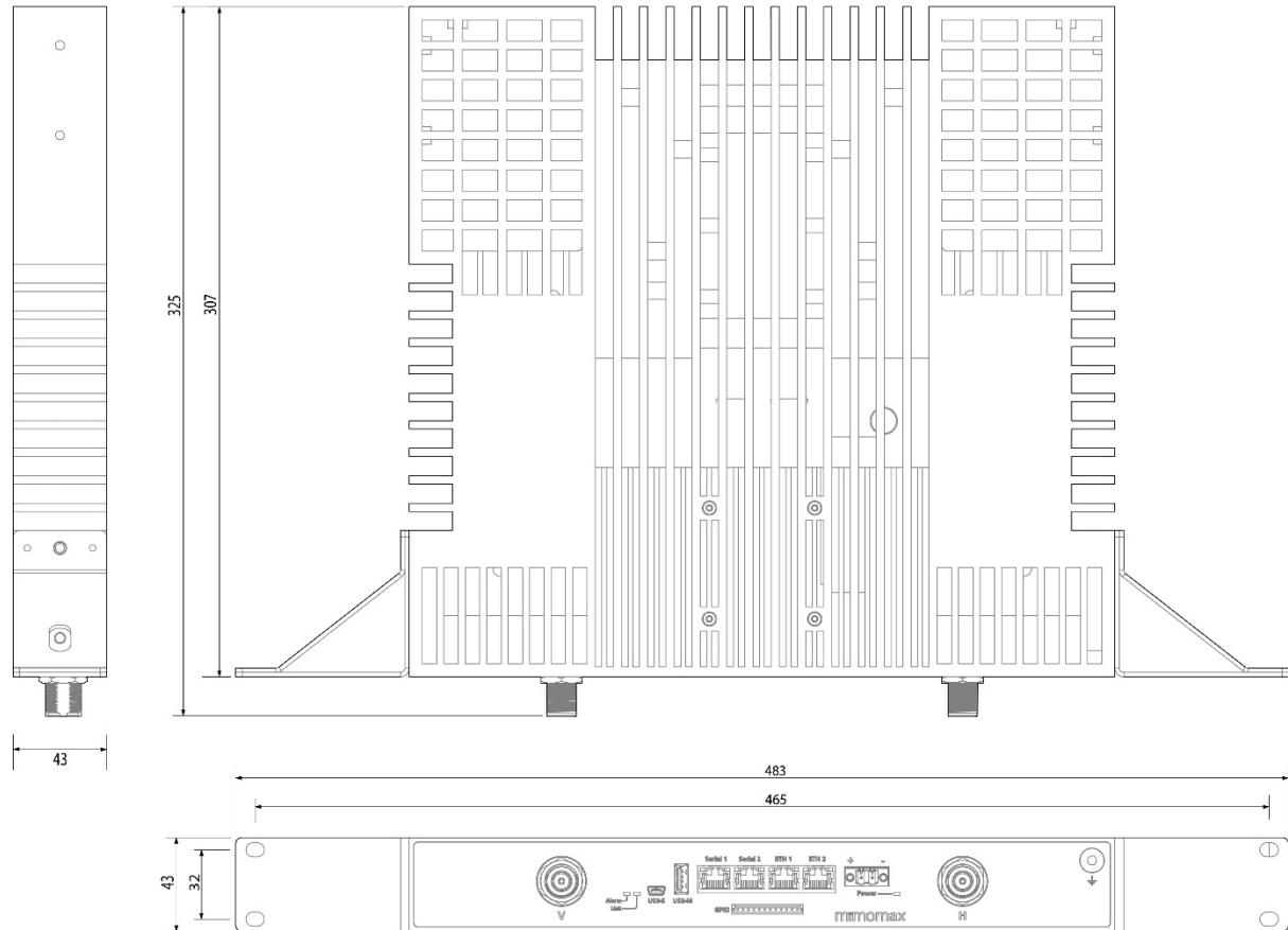
Mechanical Dimensions for Tornado X with mounting brackets (All units are in mm)
