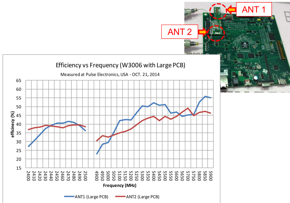
Figure 2. Antenna Efficiency
