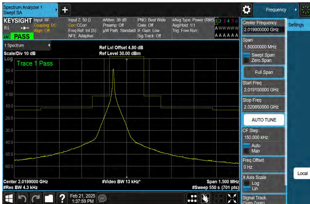
Band23-3.75kHz-MASK-HCH-QPSK-1@0
