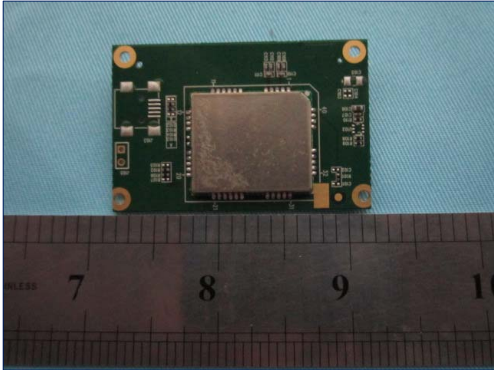
EVB Board Front View
