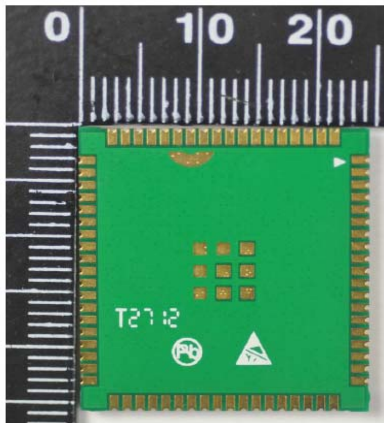
EUT – Rear View
