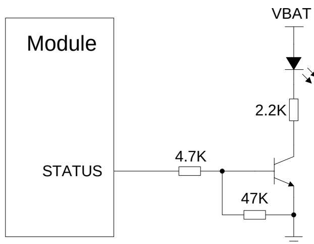
Figure 30: Reference Circuit of the STATUS
