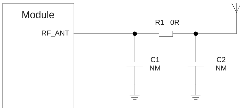
Figure 31: Reference Circuit of Antenna Interface
