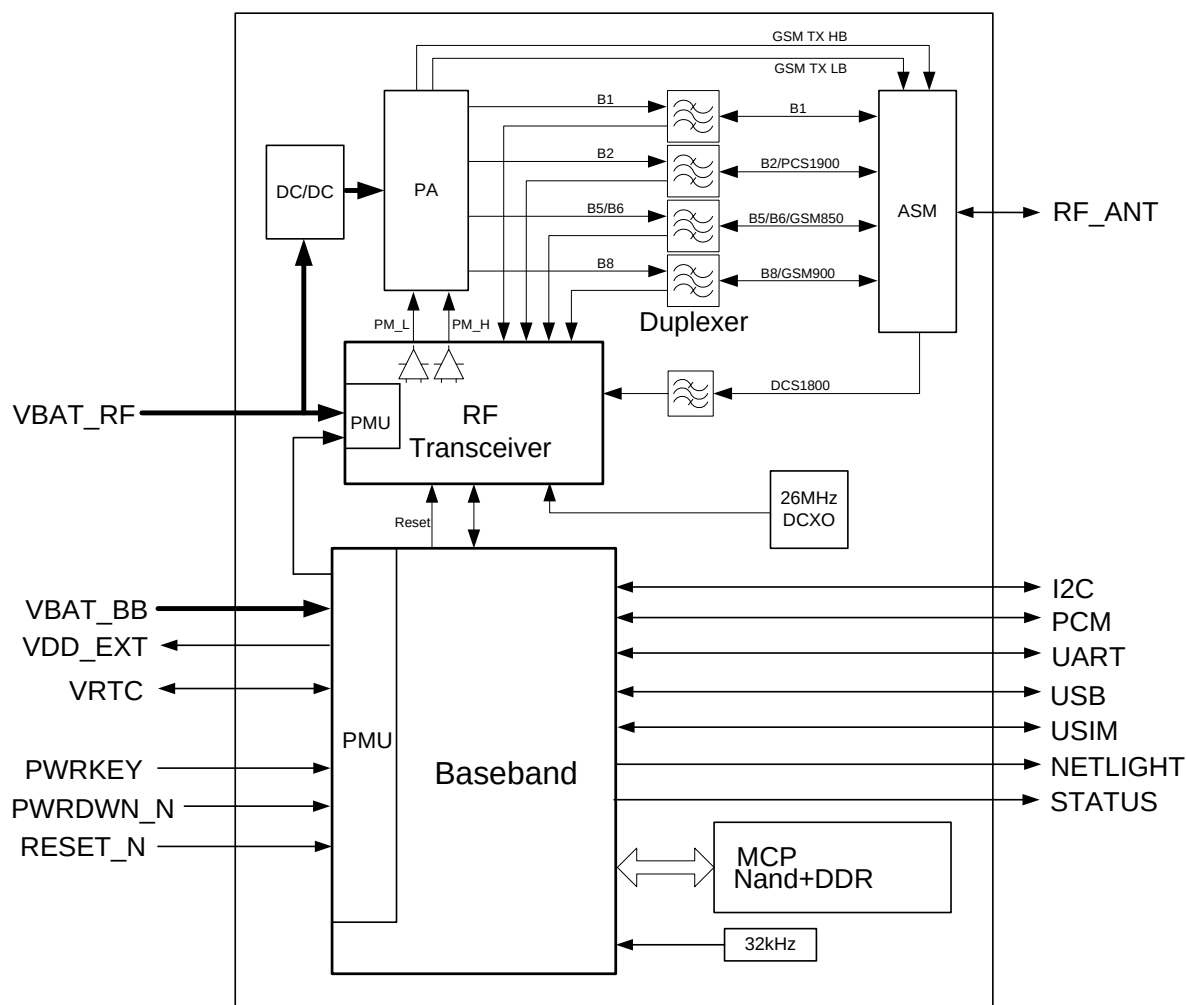
Figure 1: Functional Diagram
