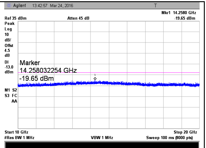
Band 2 - Low Channel-2
