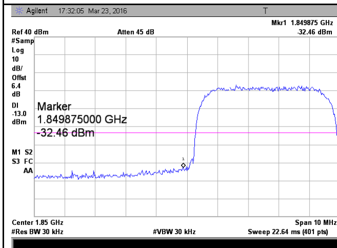
UMTS-FDD Band 2- Low Channel
