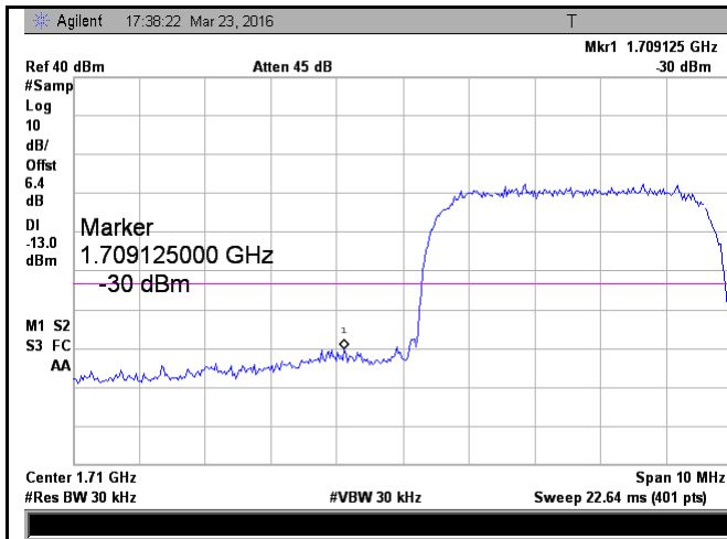
UMTS-FDD Band 4 - Low Channel
