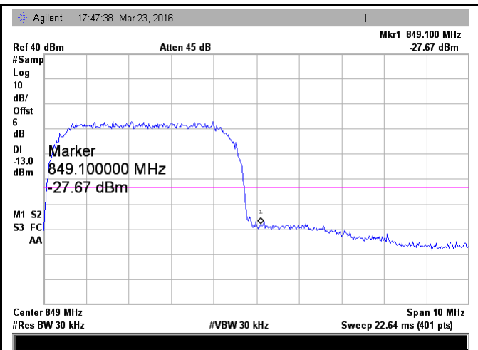
UMTS-FDD Band 5- High Channel
