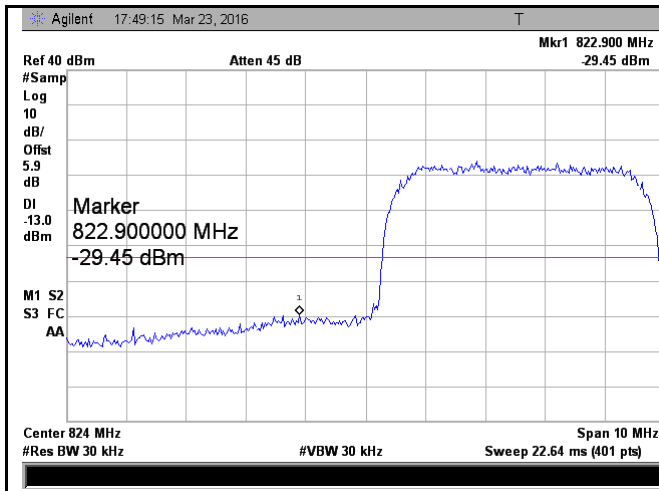
UMTS-FDD Band 5- Low Channel
