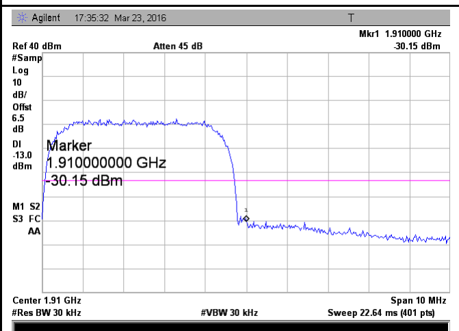
UMTS-FDD Band 2- High Channel
