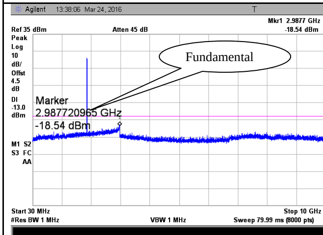
Band 2 - Middle Channel-1
