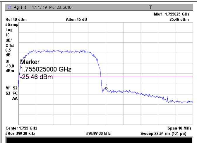
UMTS-FDD Band 4 - High Channel
