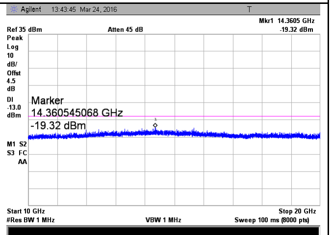
Band 2 - Middle Channel-2
