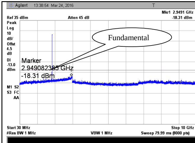
Band 2 - Low Channel-1
