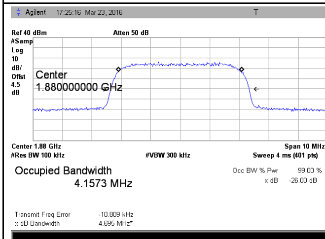
Band 2 BW - Mid CH 1880 MHz
