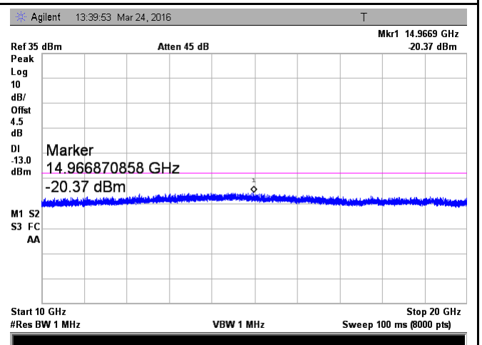
Band 2 - High Channel-2
