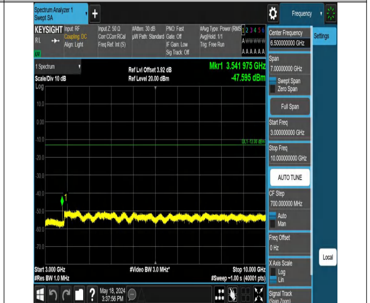
Band12_10MHz_QPSK_23060_1RB#49_3000~10000_3000~1000
