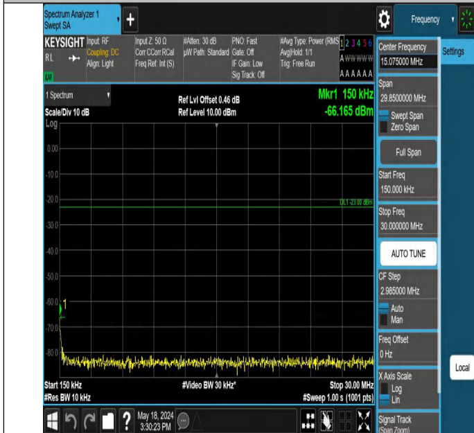
Band12_5MHz_QPSK_23035_1RB#24_0.15~30_0.15~30
