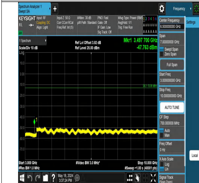
Band12_10MHz_QPSK_23060_1RB#0_3000~10000_3000~1000
