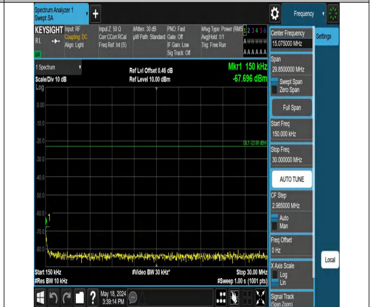
Band12_10MHz_QPSK_23130_1RB#0_0.15~30_0.15~30
