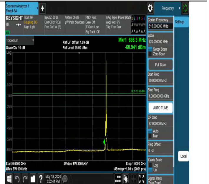
Band12_5MHz_QPSK_23155_1RB#24_30~1000_30~1000
