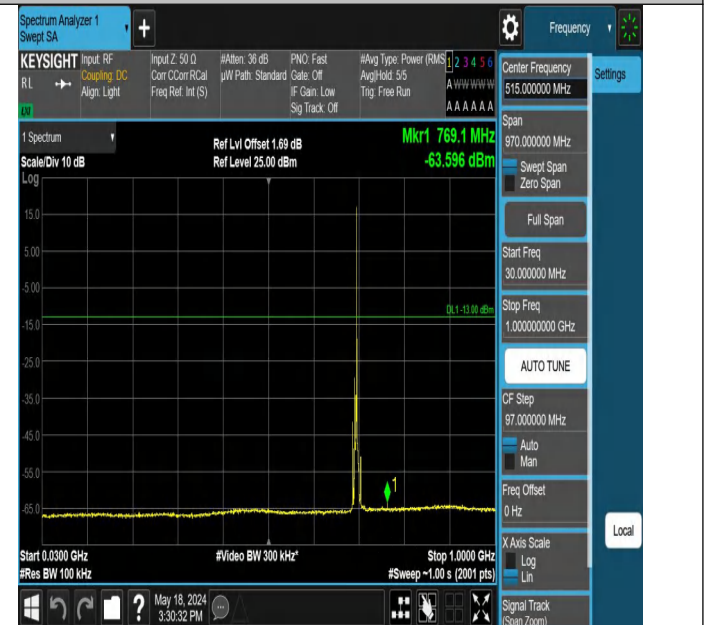
Band12_5MHz_QPSK_23035_1RB#24_30~1000_30~1000
