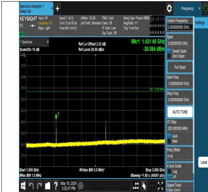
Band12_5MHz_QPSK_23155_1RB#24_1000~3000_1000~3000
