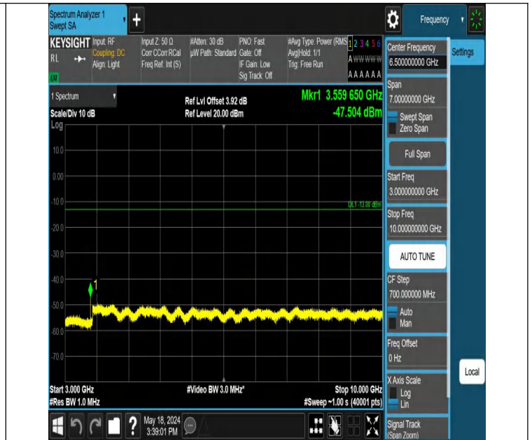
Band12_10MHz_QPSK_23095_1RB#49_3000~10000_3000~1000
