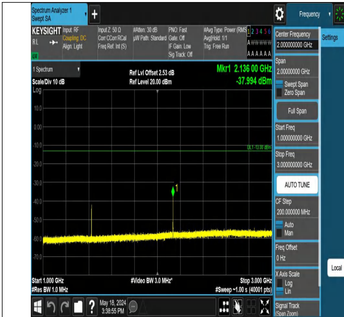
Band12_10MHz_QPSK_23095_1RB#49_1000~3000_1000~3000
