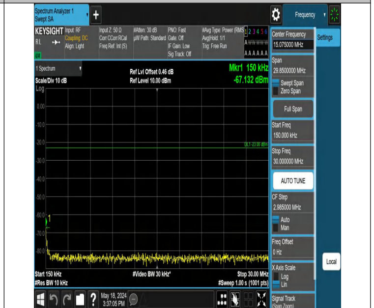
Band12_10MHz_QPSK_23060_1RB#0_0.15~30_0.15~30
