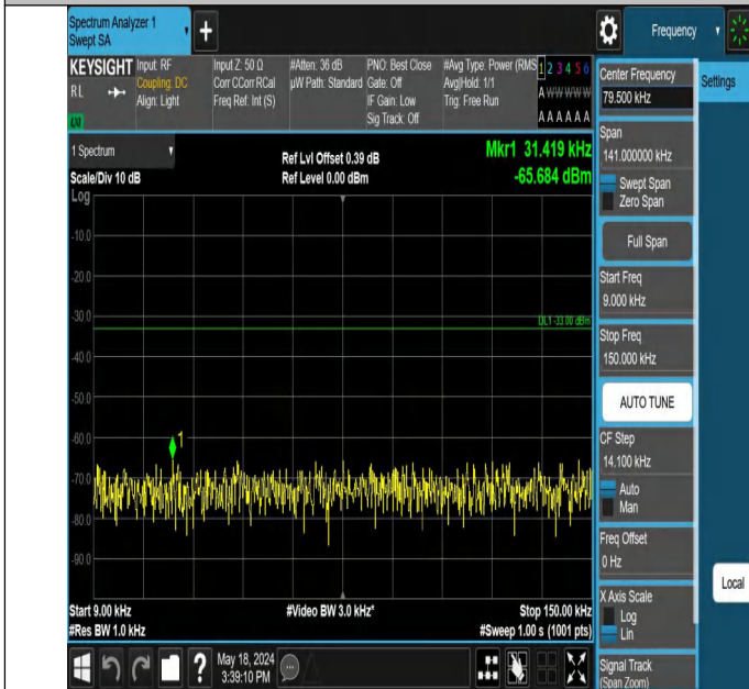
Band12_10MHz_QPSK_23130_1RB#0_0.009~0.15_0.009~0.15
