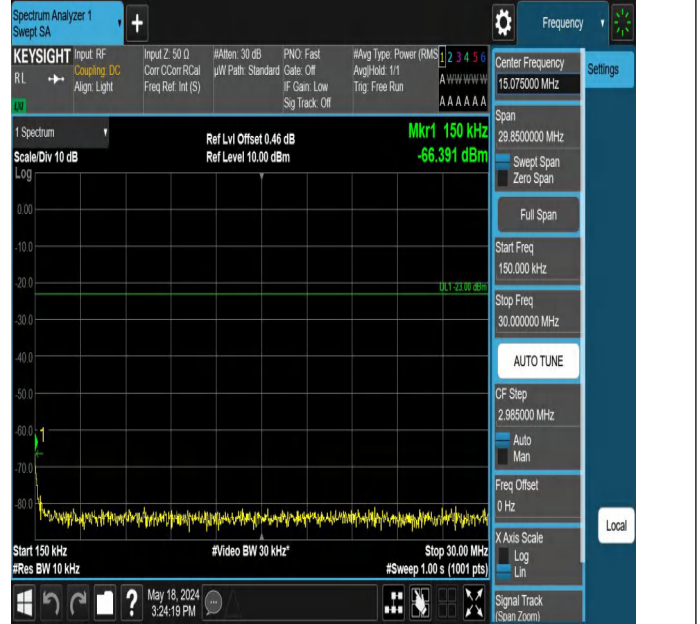
Band12_3MHz_QPSK_23165_1RB#0_0.15~30_0.15~30
