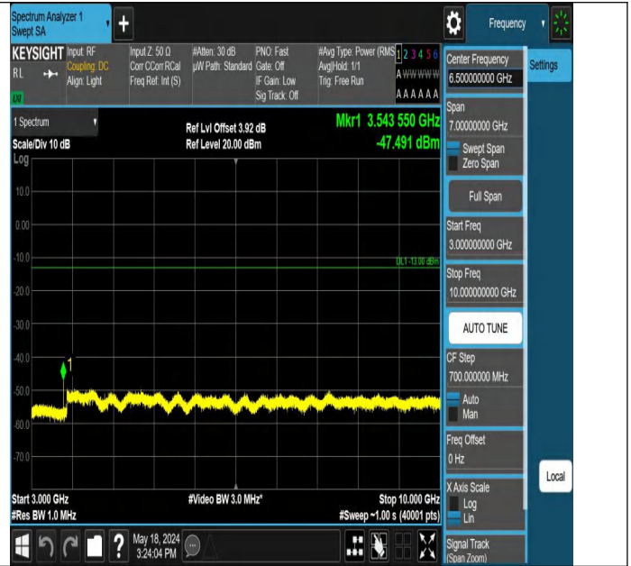
Band12_3MHz_QPSK_23095_1RB#14_3000~10000_3000~10000
