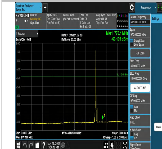
Band12_10MHz_QPSK_23095_1RB#0_30~1000_30~1000
