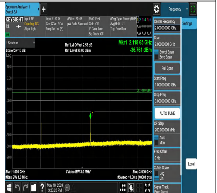
Band12_3MHz_QPSK_23095_1RB#0_1000~3000_1000~3000
