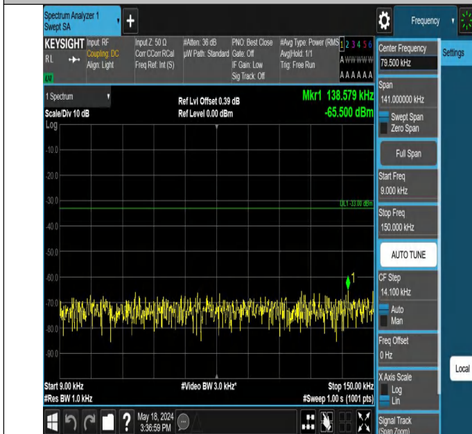
Band12_10MHz_QPSK_23060_1RB#0_0.009~0.15_0.009~0.15
