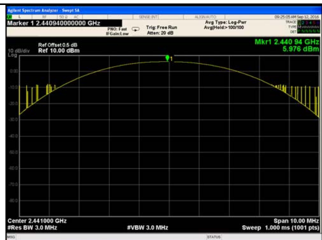
GFSK Output power - Mid CH 2441
