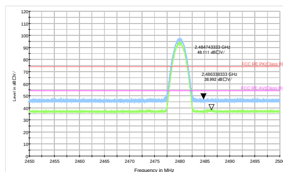
3DH5-Channel 78: Peak+ Average
