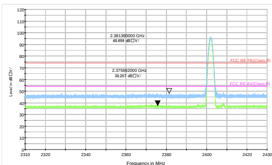
DH5-Channel 0: Peak+ Average
