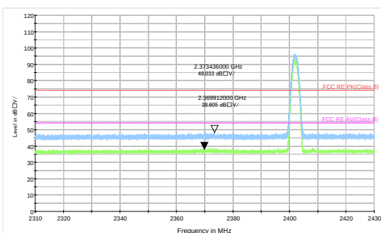
3DH5-Channel 0: Peak+ Average
