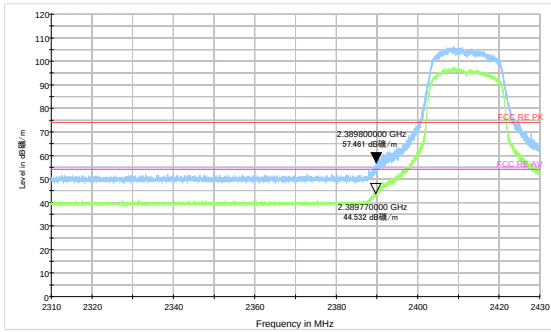
802.11n HT20 -Channel 1 Peak &amp; Average
