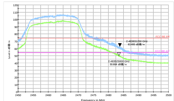
802.11g-Channel 11 Peak &amp; Average e
