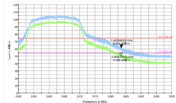
802.11g-Channel 11 Peak &amp; Average e
