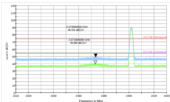
Bluetooth LE Channel 0 Peak &amp; Average
