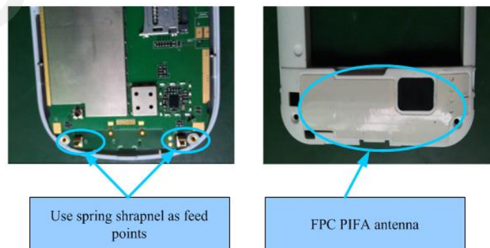
Figure 4: FPC PIFA Antenna with Spring Shrapnel as Feed Points
