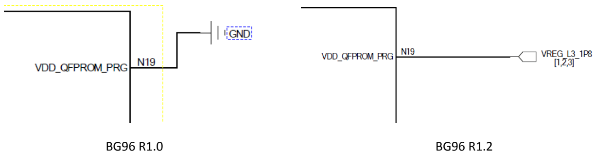
Figure 1: Schematic Designs of BG96 R1.1 and R1.2
