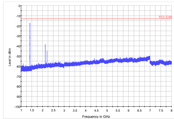
NB-IOT Band 12 CH-High 1GHz~8GHz
