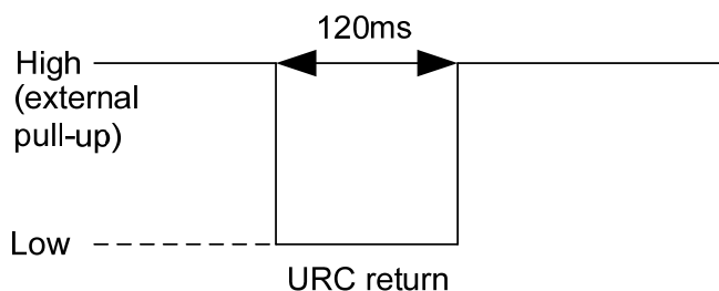
Figure 12: WAKE# Behavior
