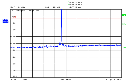
NB-IOT Band 111 CH-Middle 1GHz~3GHz
