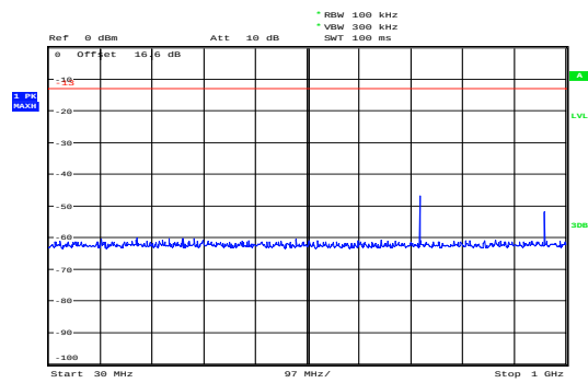
NB-IOT Band 111 CH-Middle 30MHz~1GHz
