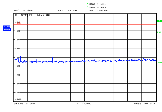
NB-IOT Band 111 CH-Middle 3GHz~20GHz
