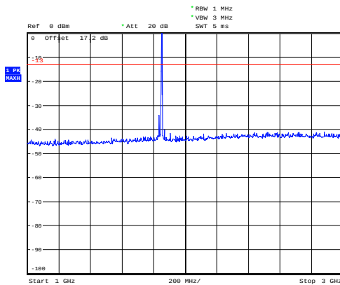
NB-IOT Band 2 CH-Low 1GHz~3GHz
