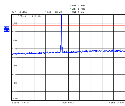
NB-IOT Band 2 CH-Middle 1GHz~3GHz
