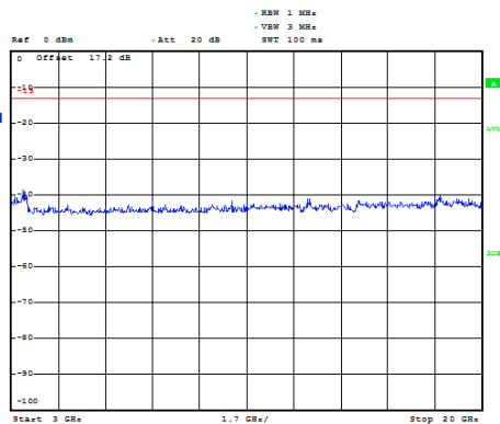
NB-IOT Band 4 CH-Low 3GHz~20GHz
