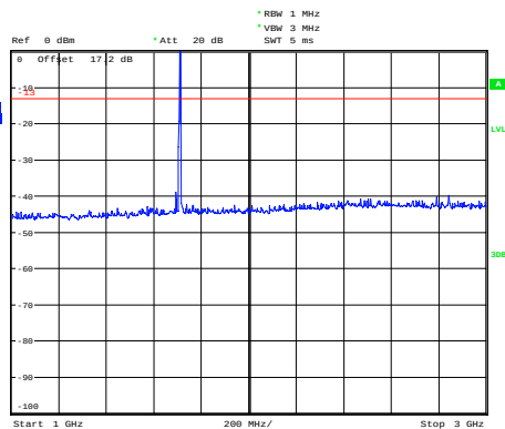
NB-IOT Band 4 CH-Low 1GHz~3GHz
