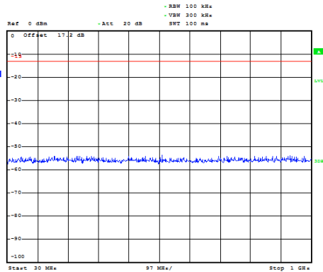
NB-IOT Band 4 CH-Low 30MHz~1GHz
