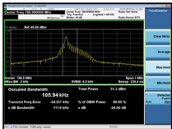
NB-IoT Band 13 QPSK 15kHz 1@0 CH-High
