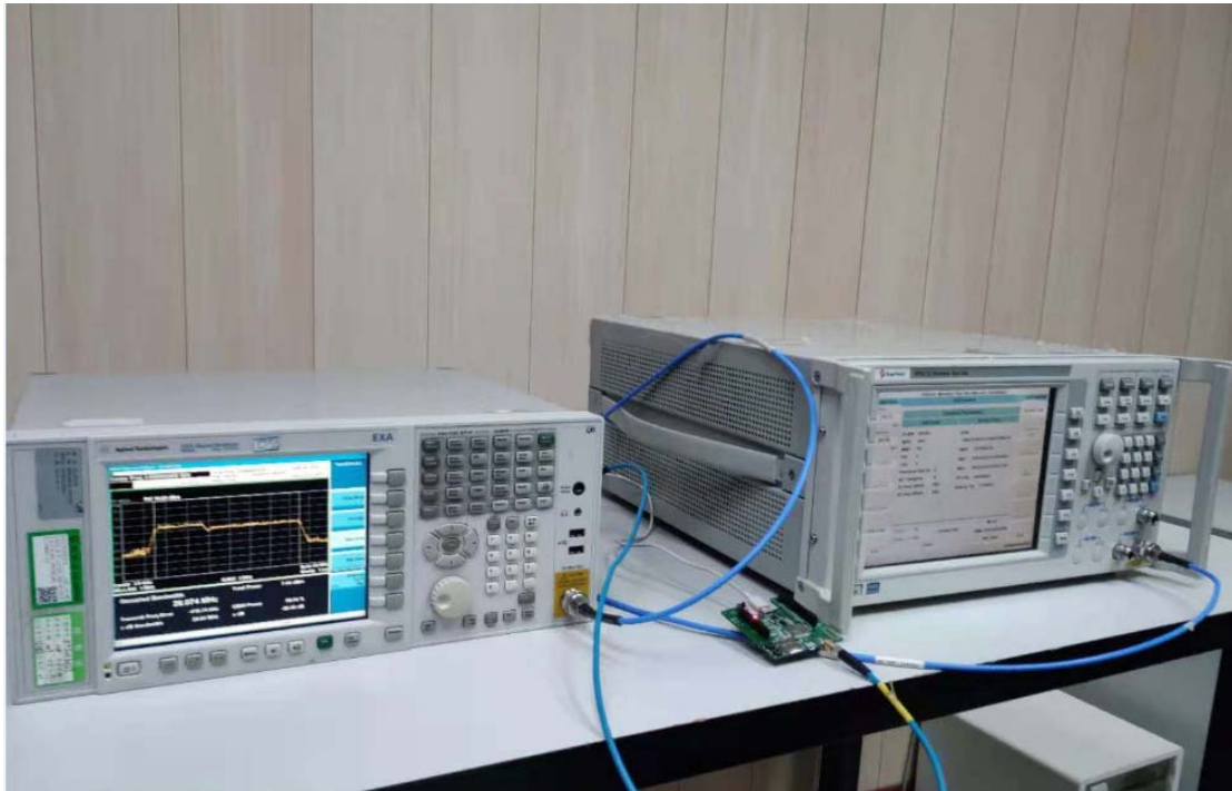
Conducted Test setup
