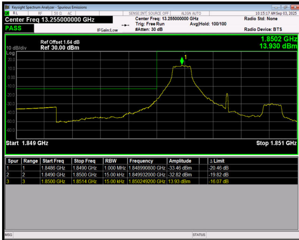
Band2 QPSK BW=1.4MHz LowChannel=18607 RB Size=6 Position=#0
