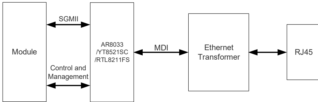
Figure 27: Simplified Block Diagram for Ethernet Application
