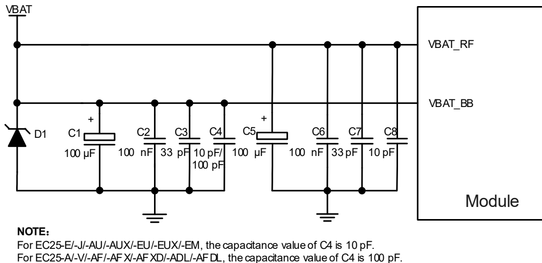
Figure 8: Star Structure of the Power Supply
