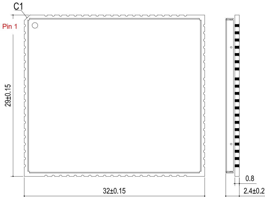
Figure 45: Module Top and Side Dimensions
