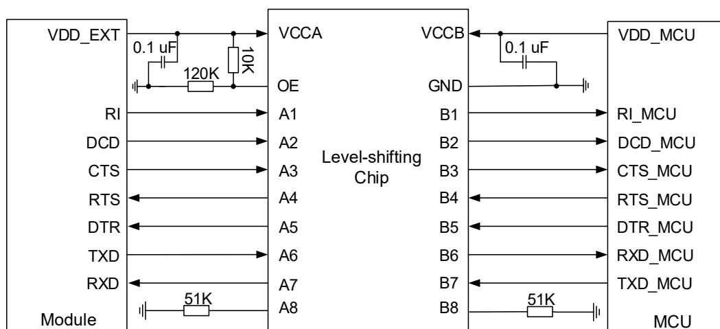
Figure 20: Reference Design of UART with Level-shifting Chip
