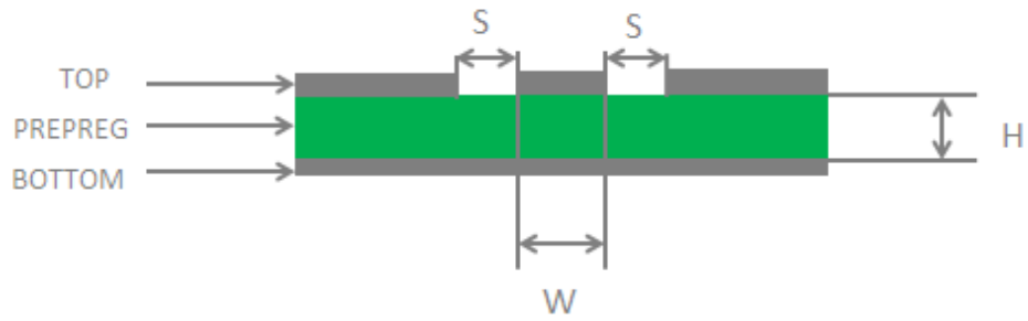
Figure 37: Coplanar Waveguide Design on a 2-layer PCB
