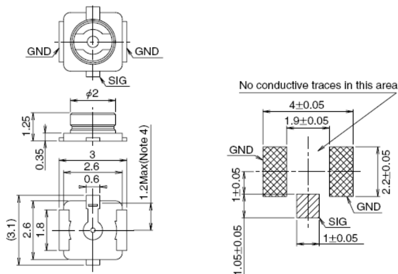
Figure 40: Dimensions of the Receptacle (Unit: mm)
