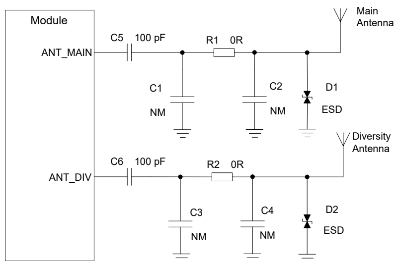
Figure 34: Reference Circuit of RF Antenna Interfaces
