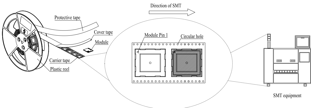
Figure 52: Mounting Direction
