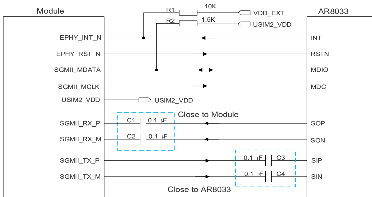
Figure 28: Reference Circuit of SGMII Interface with PHY AR8033 Application
