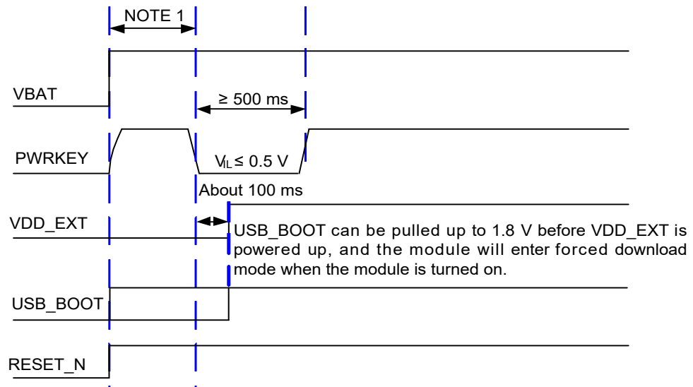
Figure 33: Timing for Entering Forced Download Mode
