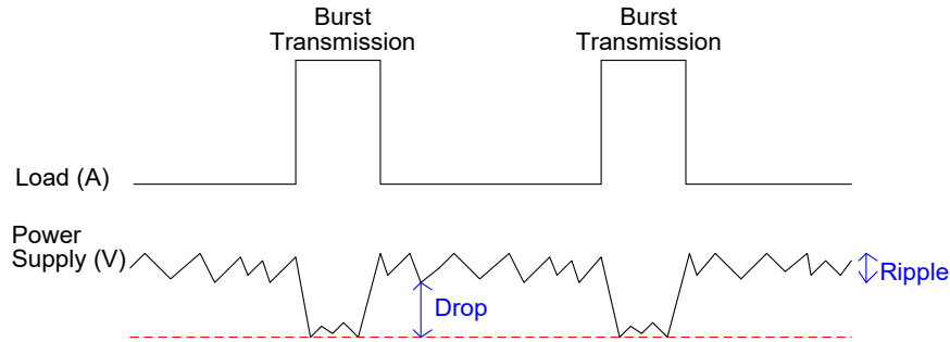
Figure 7: Power Supply Limits During Burst Transmission
