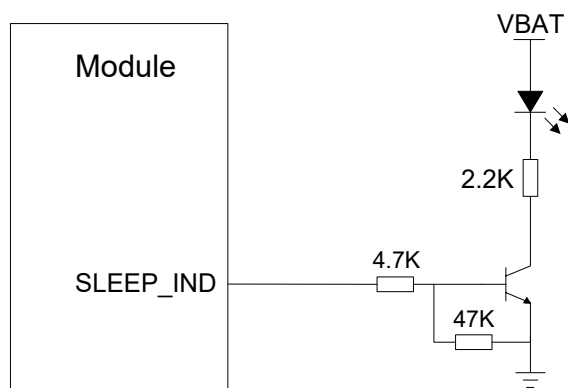
Figure 31: Reference Design of SLEEP_IND
