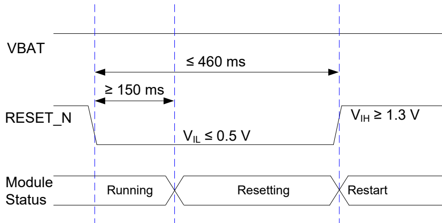
Figure 16: Reset Timing
