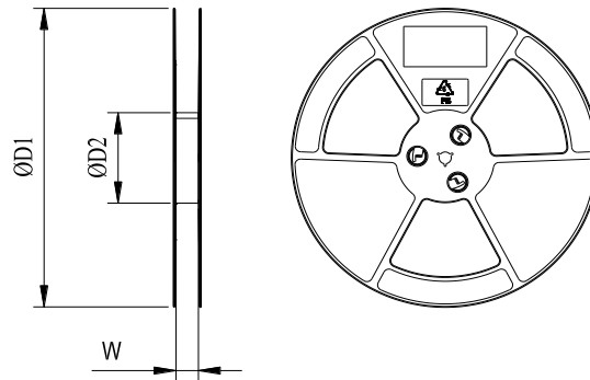
Figure 51: Plastic Reel Dimension Drawing
