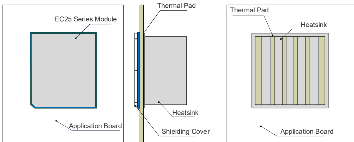
Figure 44: Referenced Heatsink Design (Heatsink at the Backside of the PCB)
