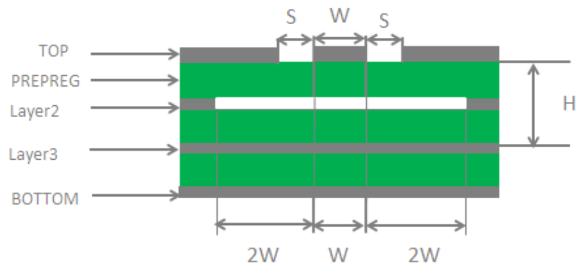
Figure 38: Coplanar Waveguide Design on a 4-layer PCB (Layer 3 as Reference Ground)
