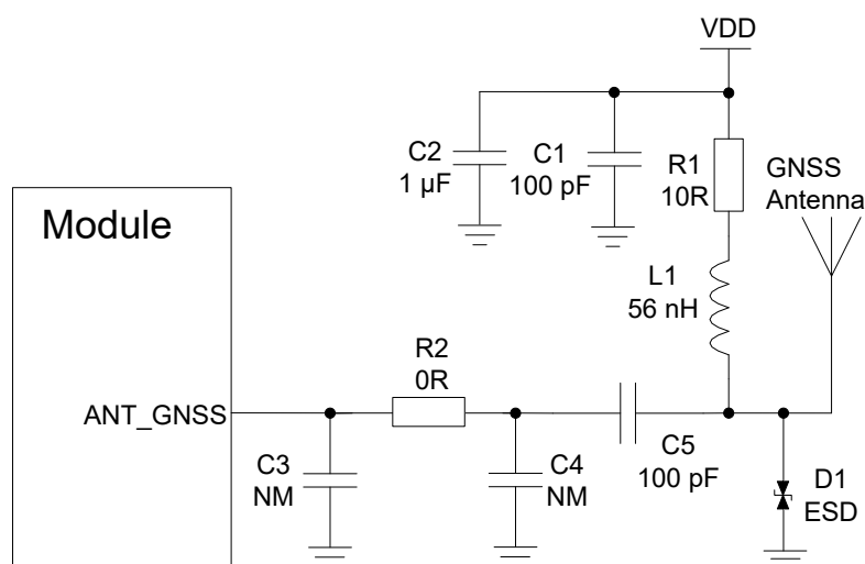
Figure 35: Reference Circuit of GNSS Antenna
