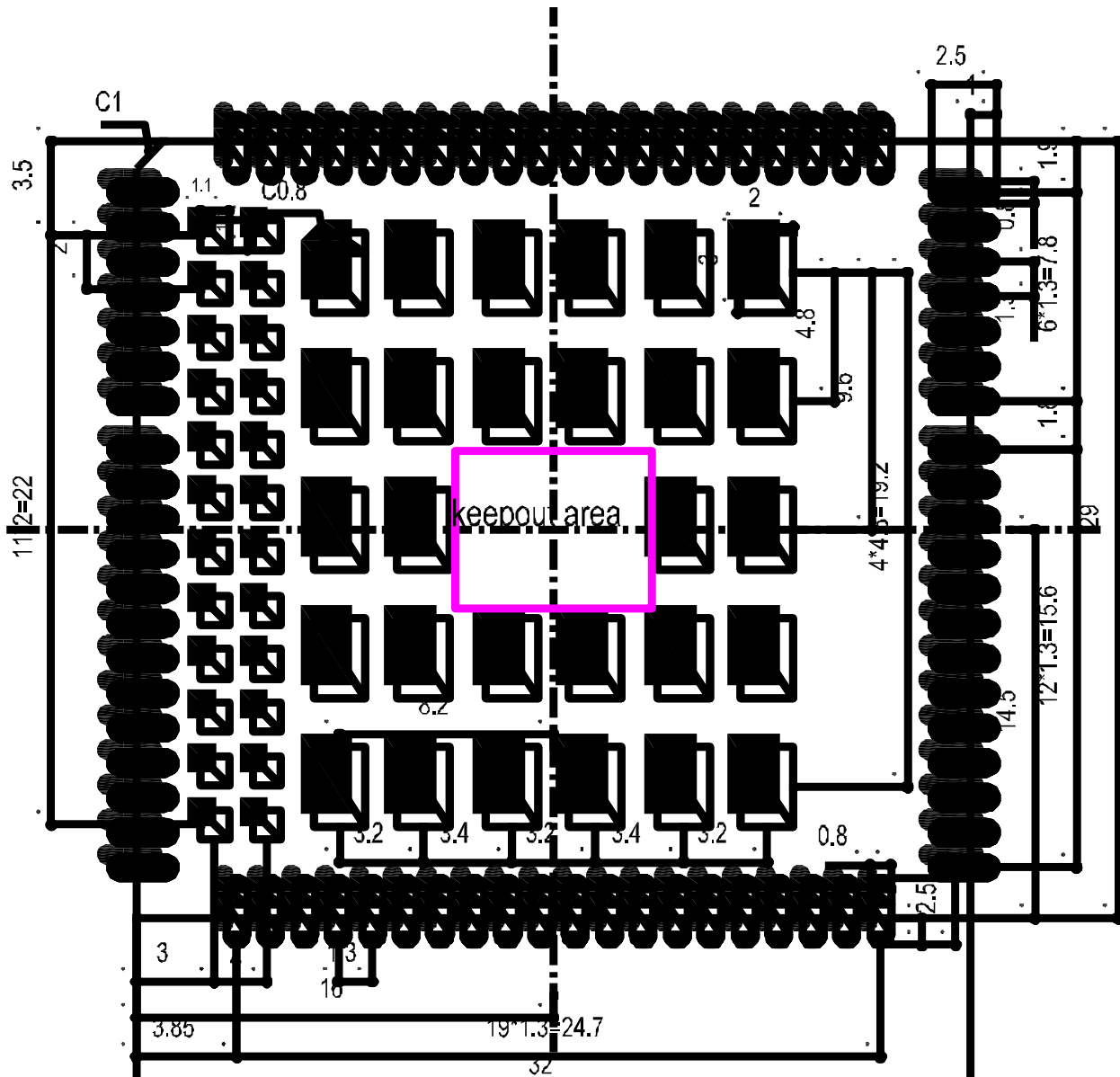
Figure 47: Recommended Footprint
