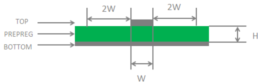
Figure 36: Microstrip Design on a 2-layer PCB
