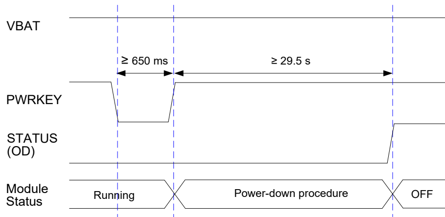
Figure 13: Turn-off Timing
