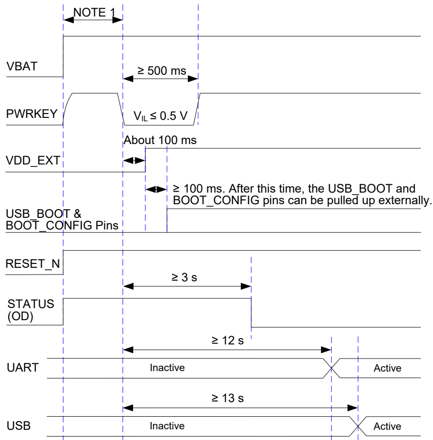
Figure 12: Turn-on Timing
