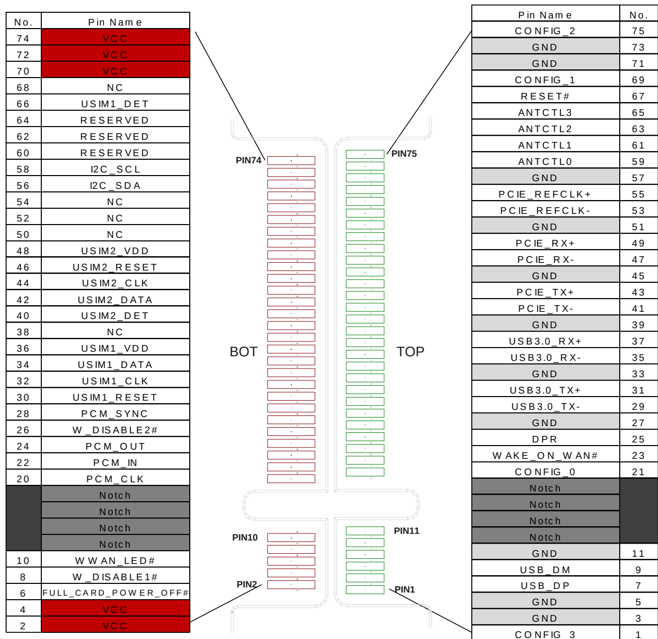
Figure 2: Pin Assignment
