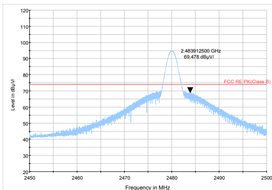
3DH5-Channel 78: Peak
