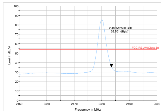
3DH5-Channel 78: Average
