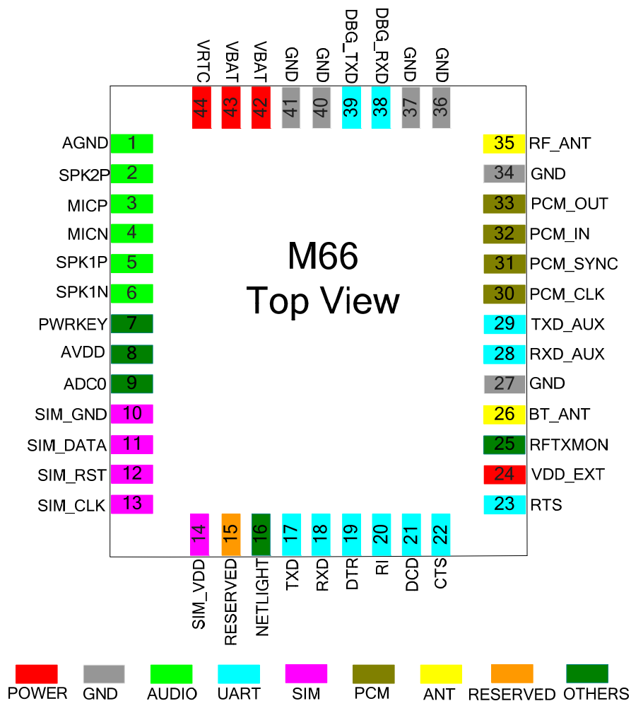
Figure 2: Pin Assignment
