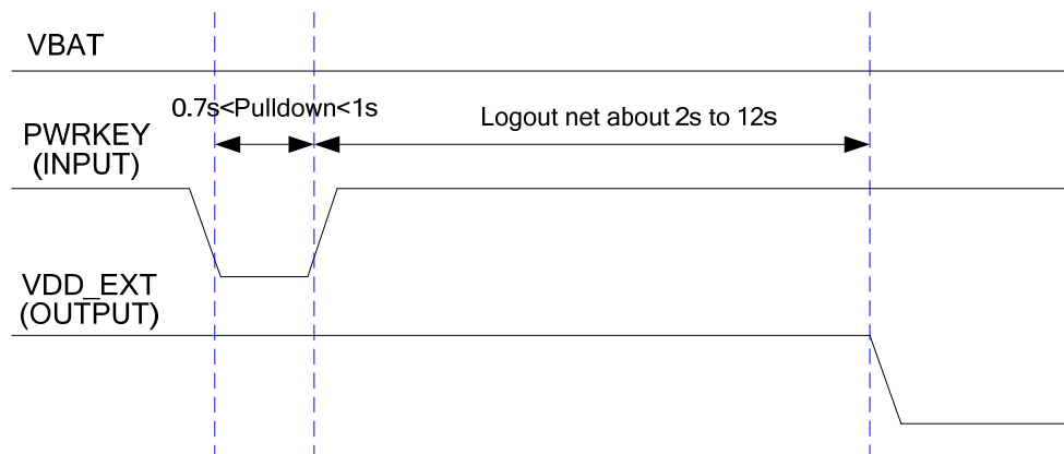
Figure 9: Turn-off Timing
