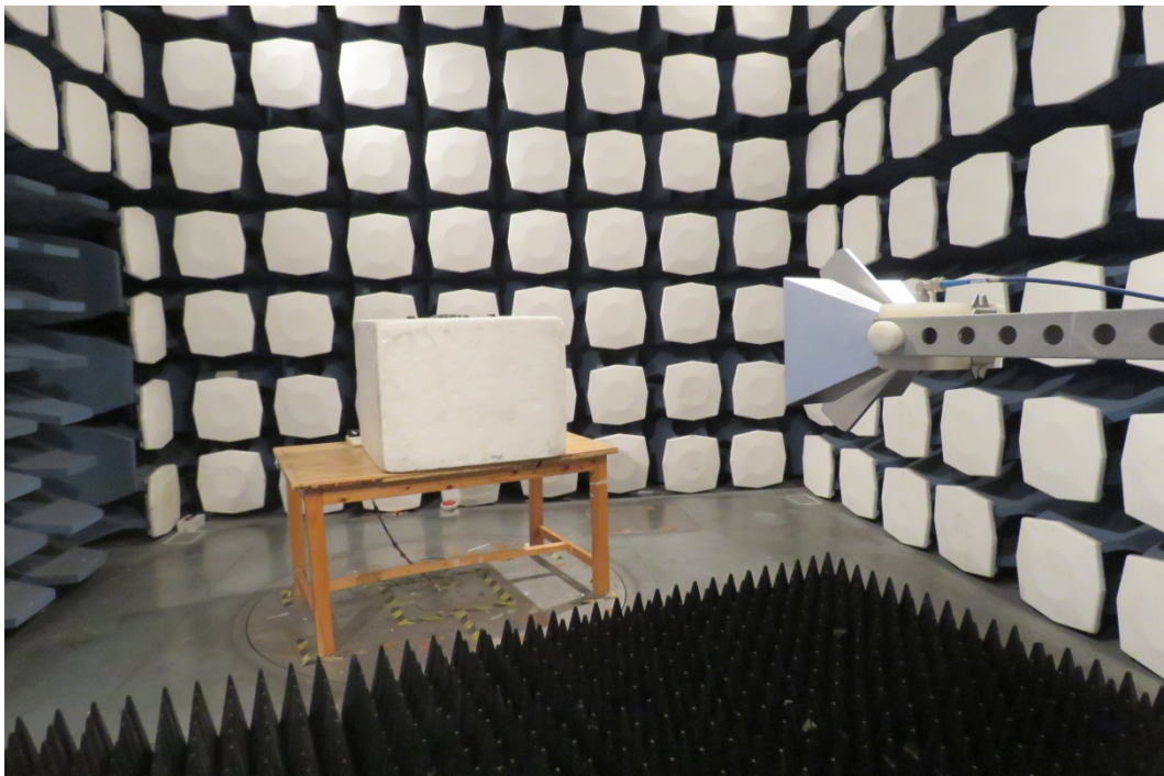
Radiated Spurious Emissions Test setup
