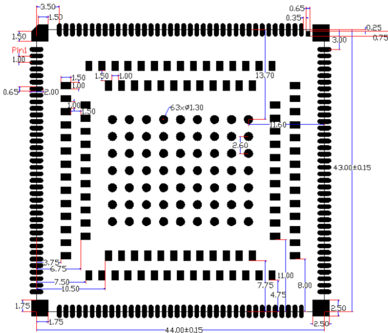
Figure 47: Recommended Footprint (Top View)
