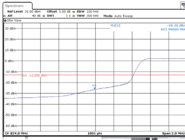
BAND5_10MHz_16QAM_20450_50RB#0
