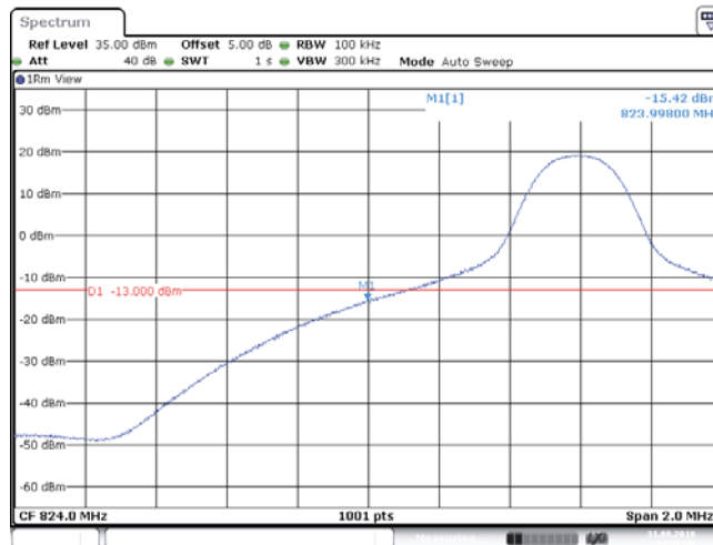
BAND5_10MHz_64QAM_20450_50RB#0
