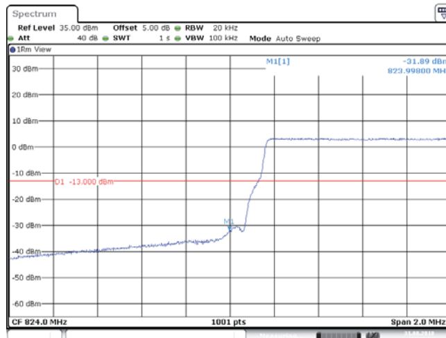
BAND5_1.4MHz_64QAM_20407_6RB#0
