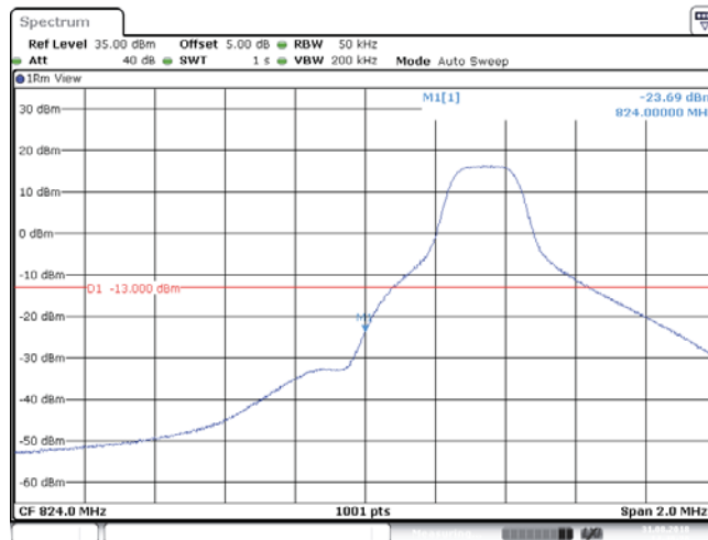
BAND5_5MHz_64QAM_20425_25RB#0
