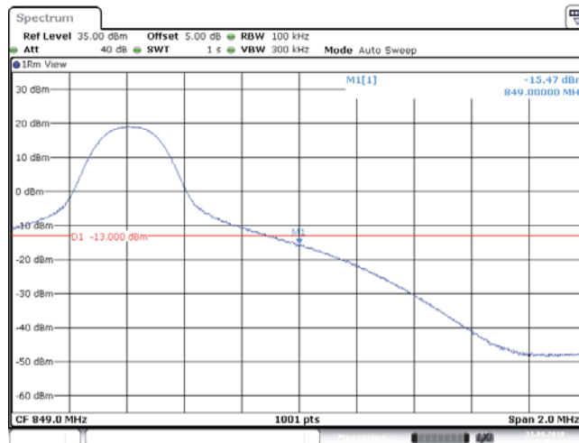
BAND5_10MHz_64QAM_20600_50RB#0
