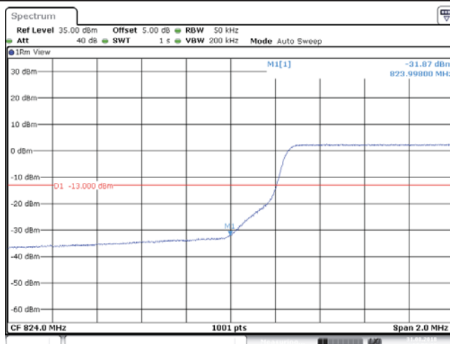
BAND5_5MHz_16QAM_20425_25RB#0
