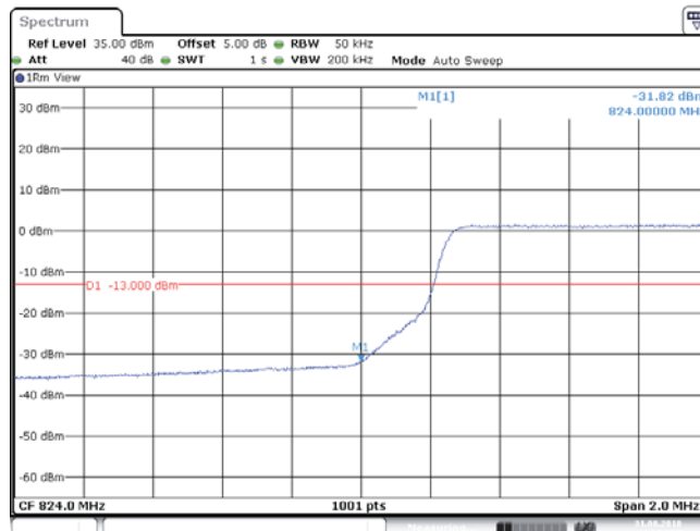
BAND5_5MHz_64QAM_20425_25RB#0
