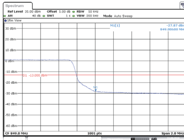
BAND5_5MHz_64QAM_20625_25RB#0
