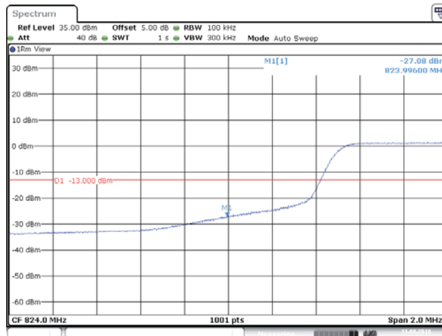
BAND5_10MHz_64QAM_20450_50RB#0
