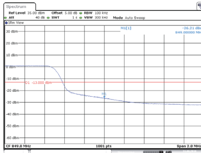
BAND5_10MHz_64QAM_20600_50RB#0
