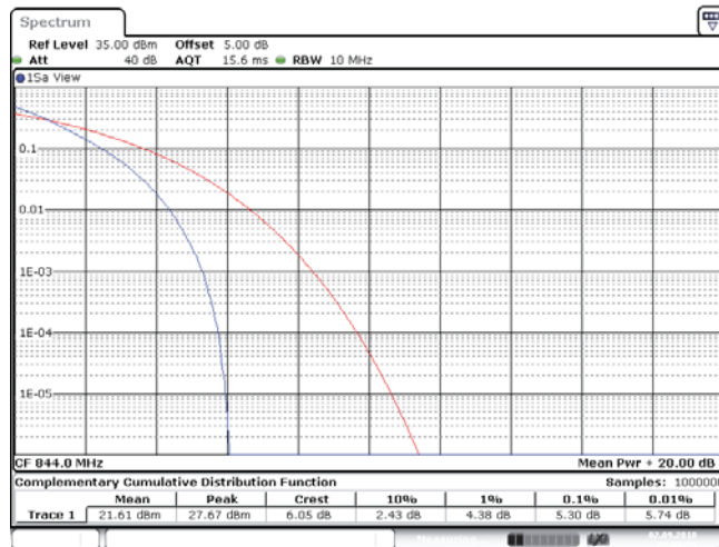
BAND5_10MHz_QPSK_20600_50RB#0
