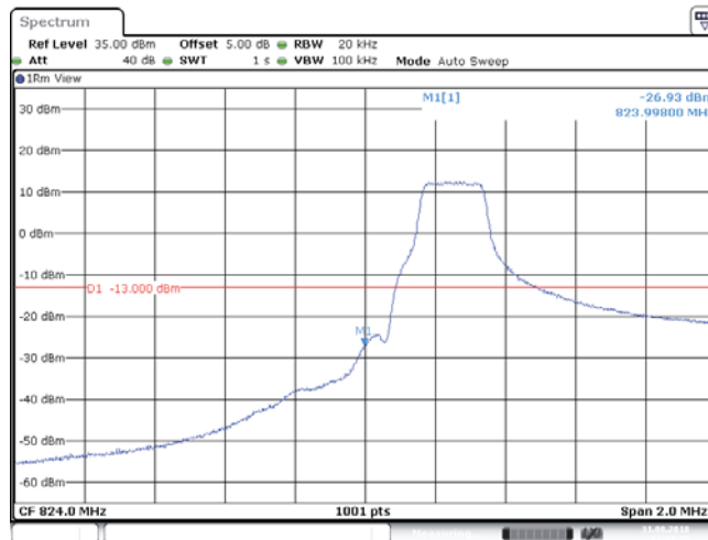
BAND5_1.4MHz_64QAM_20407_6RB#0
