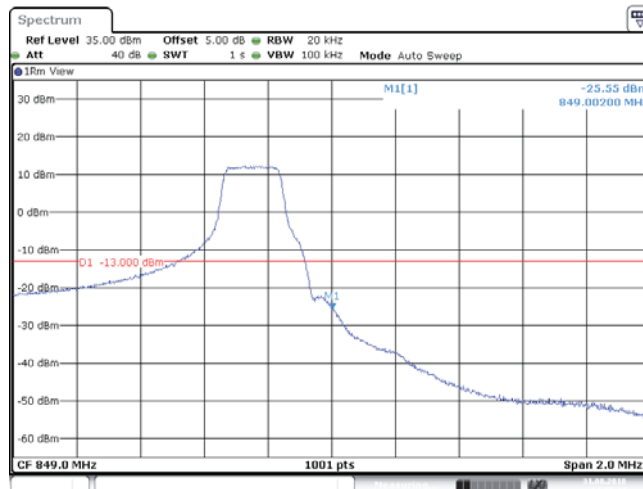
BAND5_1.4MHz_64QAM_20643_6RB#0
