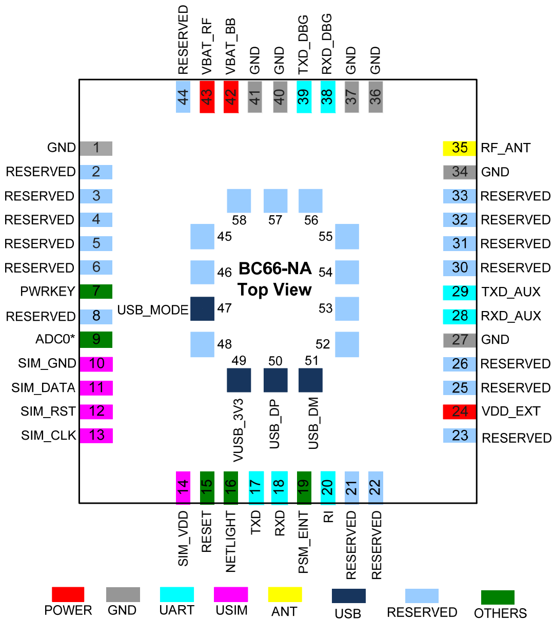
Figure 2: Pin Assignment
