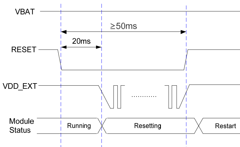
Figure 14: Reset Timing
