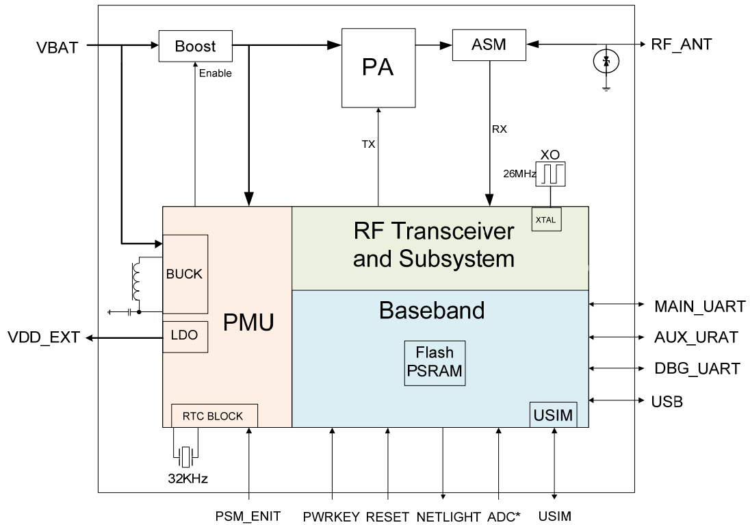
Figure 1: Functional Diagram
