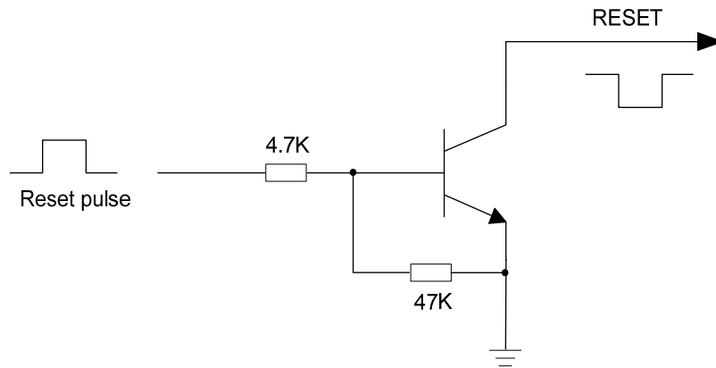
Figure 12: Reference Circuit of RESET by Using Driving Circuit
