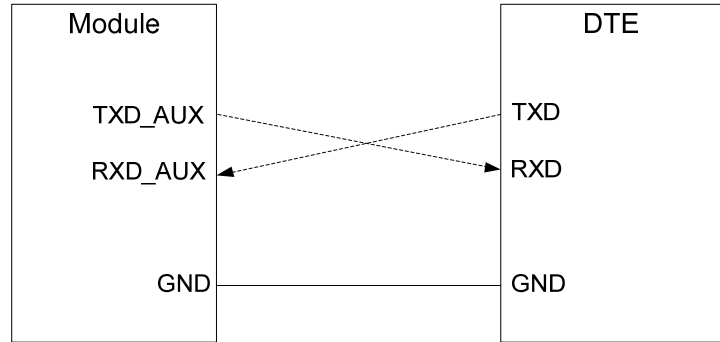
Figure 18: Reference Design of Auxiliary UART Port
