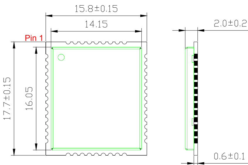
Figure 31: BC66-NA Top and Side Dimensions (Unit: mm)
