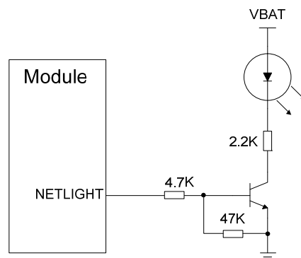
Figure 24: Reference Design of NETLIGHT
