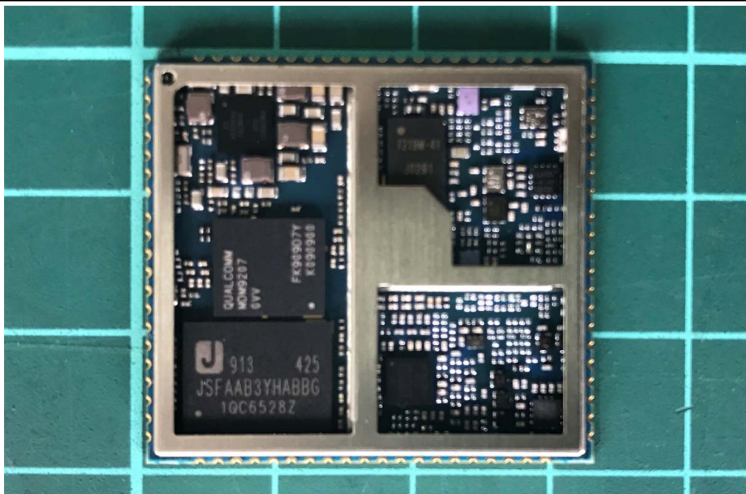
Picture 1 EUT
