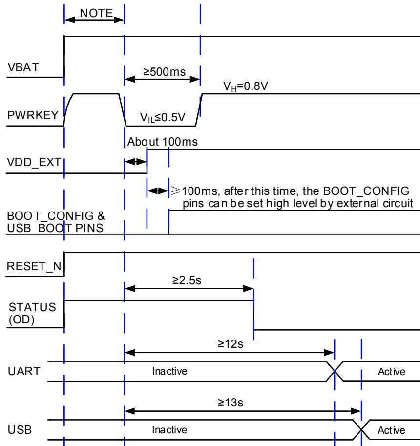
Figure 12: Power-on Scenario of Module
