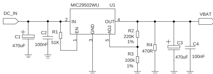
Figure 5: Reference Circuit of Power Supply
