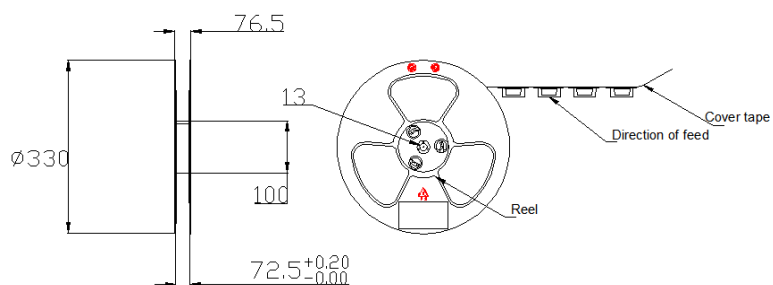
Figure 55: Reel Dimensions
