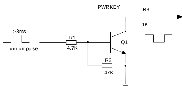
Figure 6: Turn on the Module Using Driving Circuit
