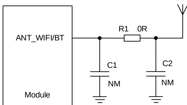
Figure 41: Reference Circuit Design for Wi-Fi/BT Antenna Interface
