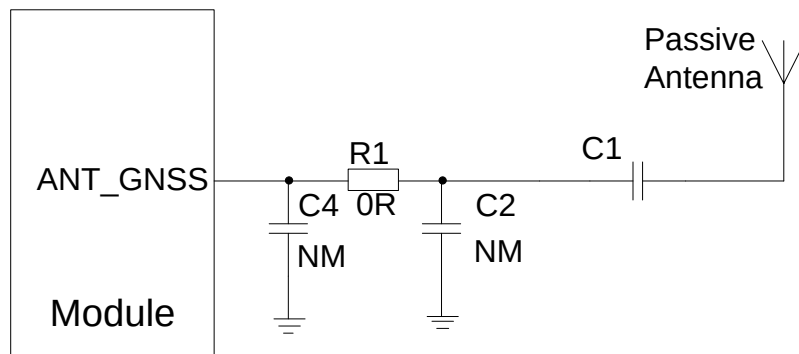
Figure 43: Reference Circuit Design for GNSS Passive Antenna
