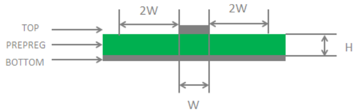
Figure 37: Microstrip Design on a 2-layer PCB
