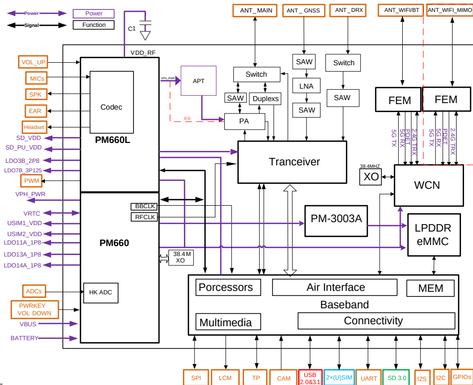
Figure 1: Functional Diagram
