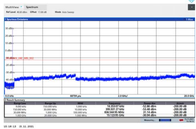
GPRS 850 CH-High 9kHz ~ 20GHz
