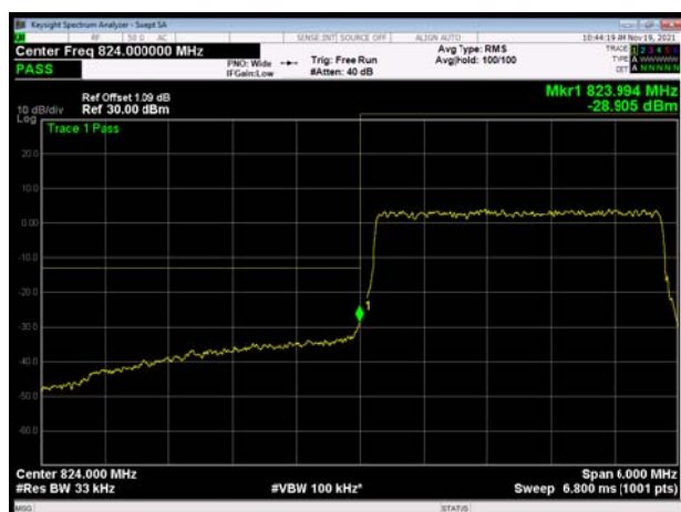
LTE Band 5 5MHz 16QAM 1RB CH-Low
