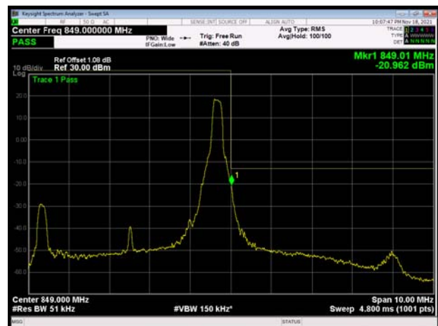
LTE Band 5 5MHz QPSK 1RB CH-High
