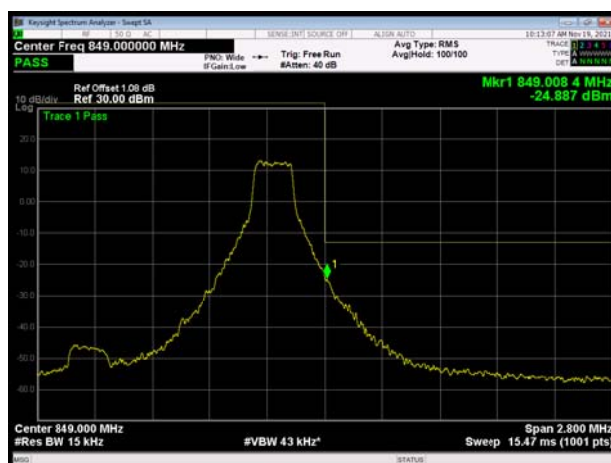
LTE Band 5 1.4MHz 16QAM 100%RB CH-High
