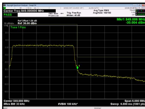
LTE Band 5 5MHz 16QAM 1RB CH-High
