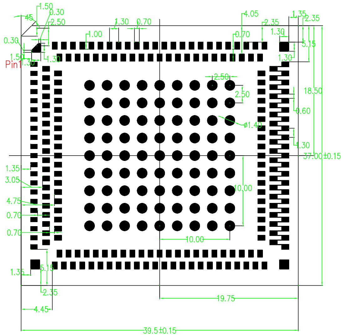
Figure 45: Module Bottom Dimensions (Top View)
