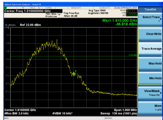
GSM 1900 GPRS CH-High
