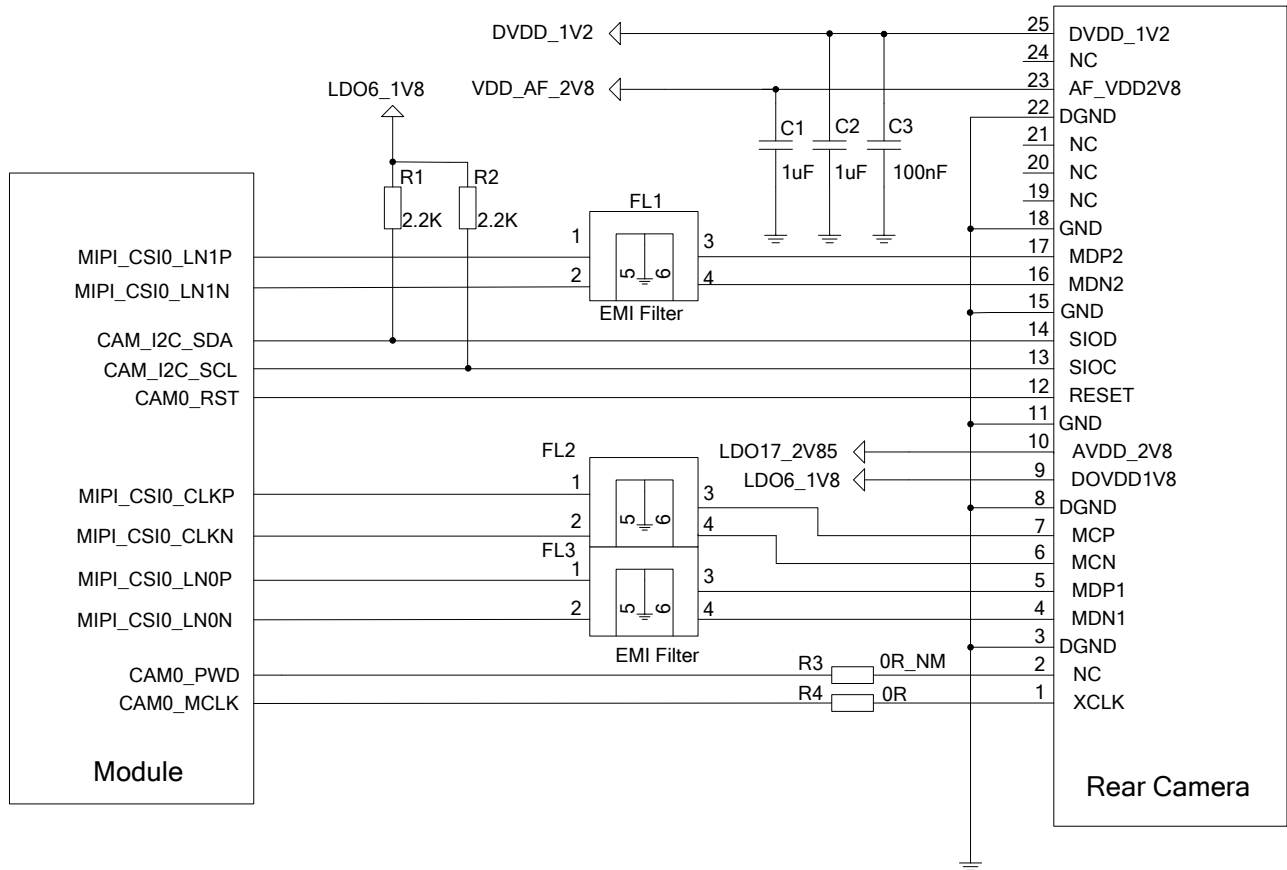
Figure 22: Reference Circuit Design for Rear Camera Interface
