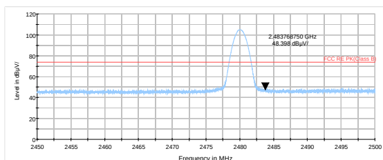
3DH5-Channel 78: Peak
