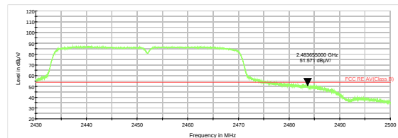
802.11n HT40 -Channel 9 Average
