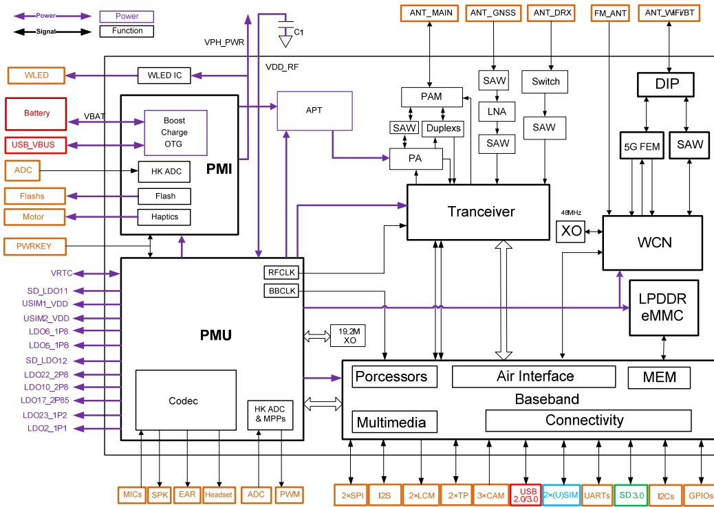
Figure 1: Functional Diagram
