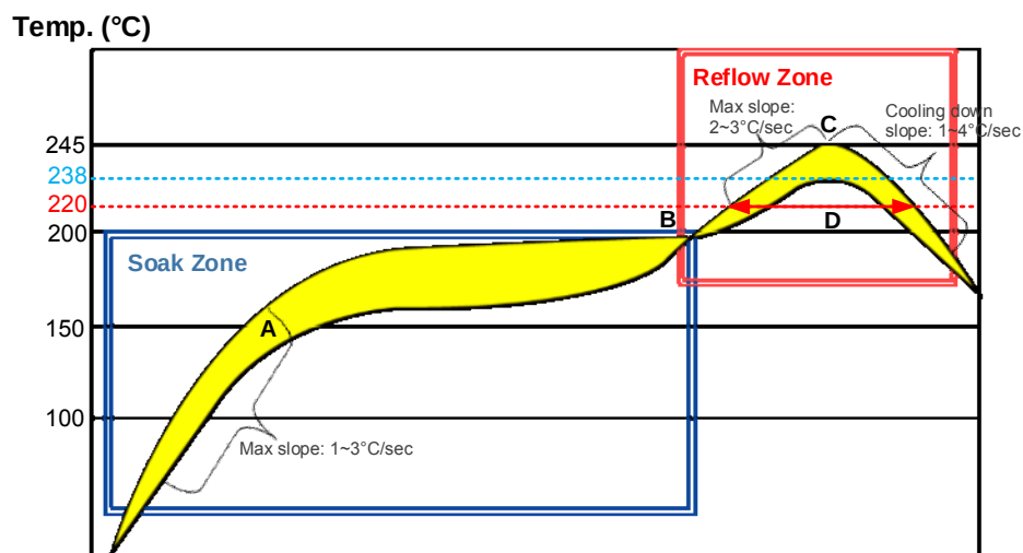
Figure 45: Recommended Reflow Soldering Thermal Profile
