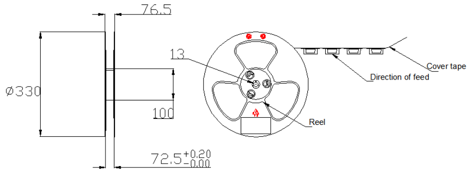
Figure 47: Reel Dimensions
