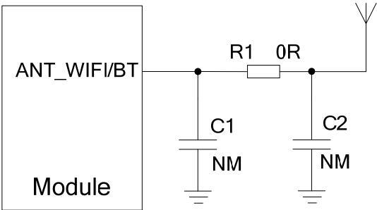
Figure 33: Reference Circuit Design for Wi-Fi/BT Antenna Interface
