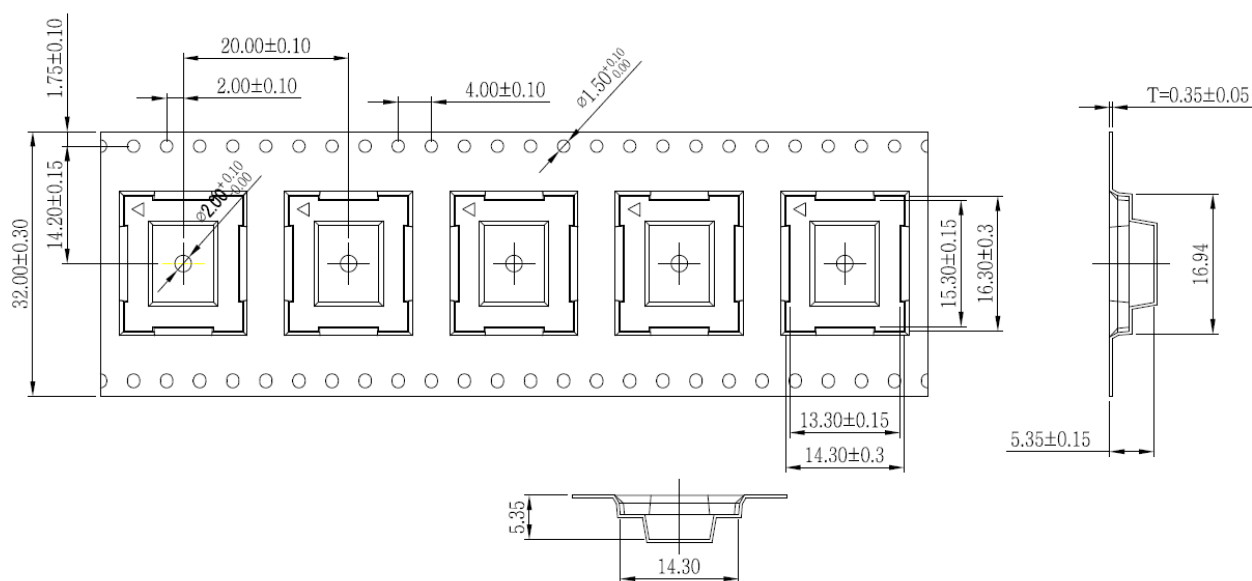
Figure 38: Tape Dimensions
