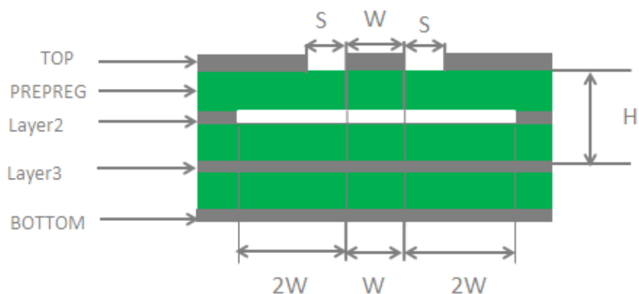
Figure 26: Coplanar Waveguide Line Design on a 4-layer PCB (Layer 3 as Reference Ground)
