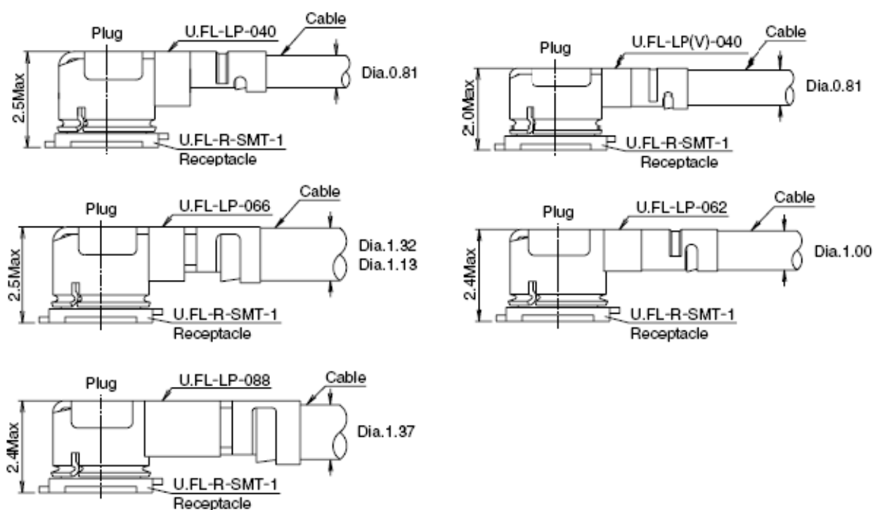
Figure 31: Space Factor of Mated Connector (Unit: mm)
